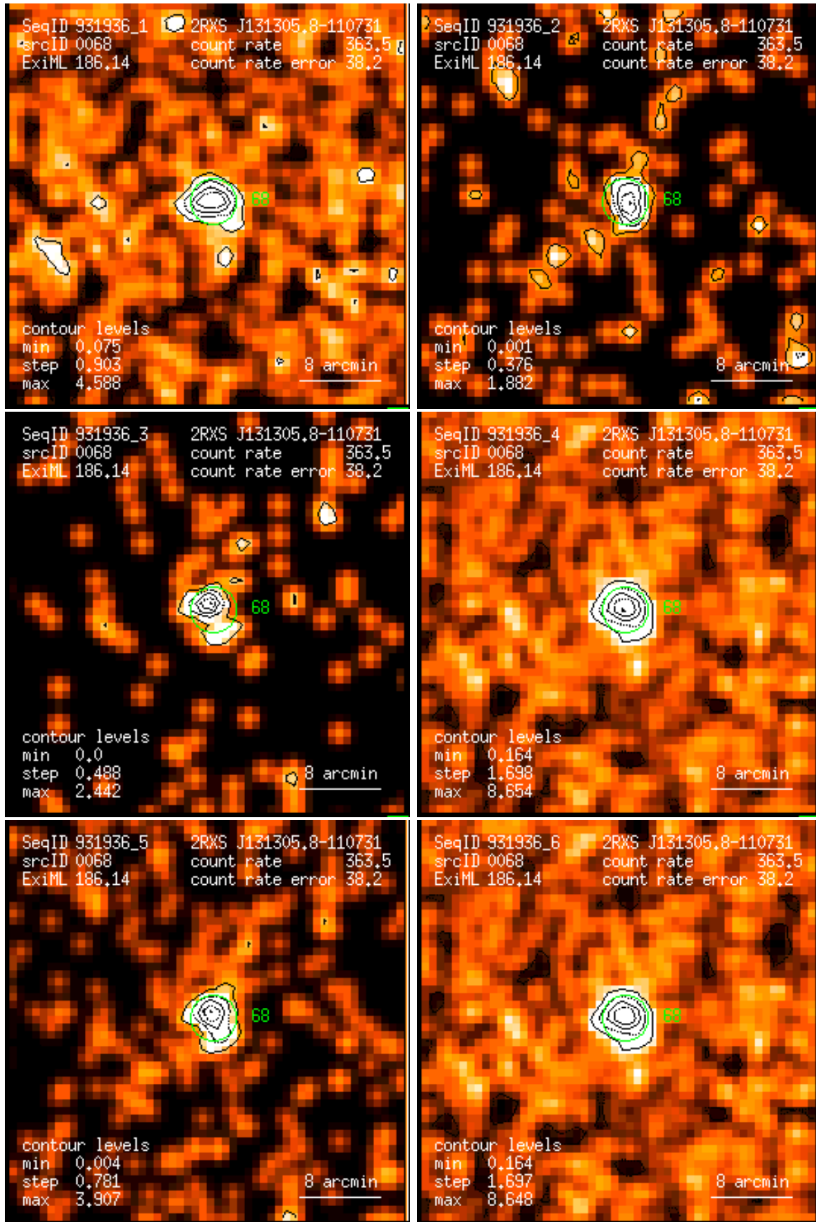
Figure 68: RASS 931936: detection 0068: band rate images, Gaussian filter: (1) PSPC channels 11 – 41, (2) 52 – 90, (3) 91 – 201, (4) 11 – 235, (5) 52 – 201, (6) 11 – 201. Broad band rates in counts/ks. Band rate contour levels in counts/ks/arcmin 2 .
