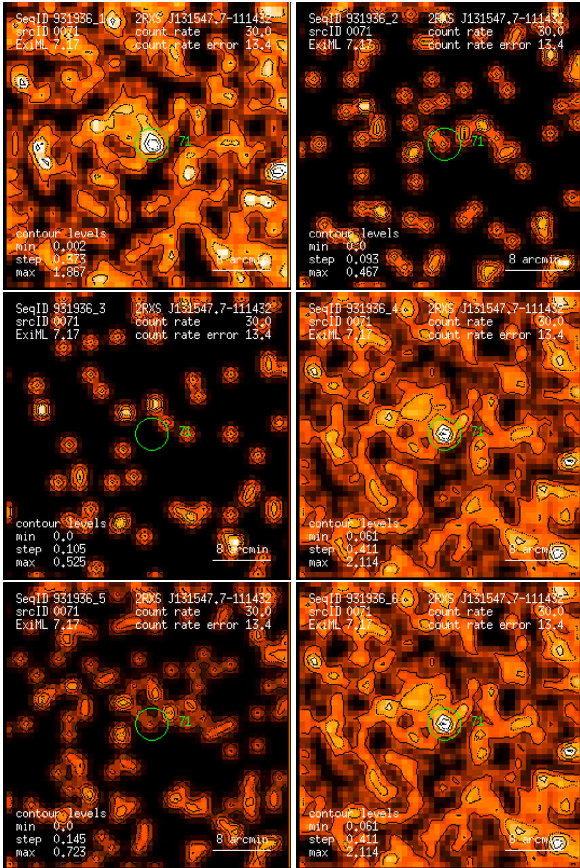
Figure 71: RASS 931936: detection 0071: band rate images, Gaussian filter: (1) PSPC channels 11 – 41, (2) 52 – 90, (3) 91 – 201, (4) 11 – 235, (5) 52 – 201, (6) 11 – 201. Broad band rates in counts/ks. Band rate contour levels in counts/ks/arcmin 2 .
