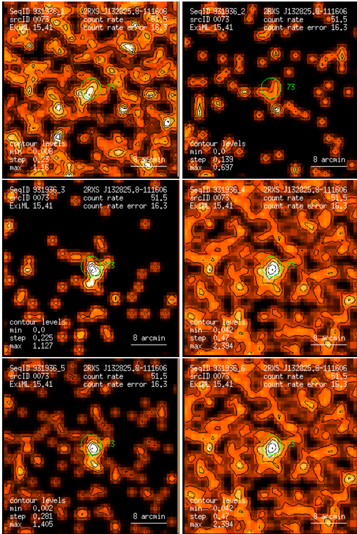
Figure 73: RASS 931936: detection 0073: band rate images, Gaussian filter: (1) PSPC channels 11 – 41, (2) 52 – 90, (3) 91 – 201, (4) 11 – 235, (5) 52 – 201, (6) 11 – 201. Broad band rates in counts/ks. Band rate contour levels in counts/ks/arcmin 2 .
