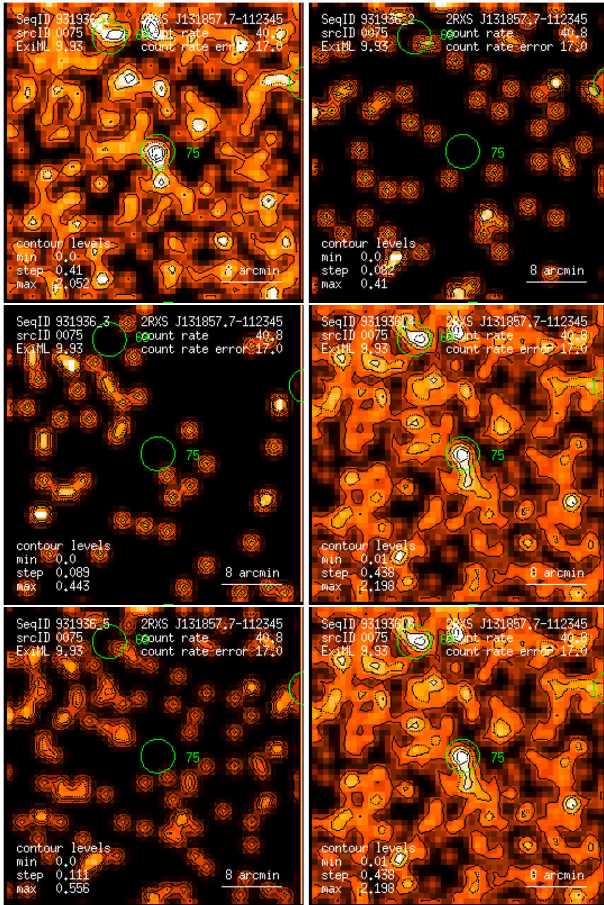
Figure 75: RASS 931936: detection 0075: band rate images, Gaussian filter: (1) PSPC channels 11 – 41, (2) 52 – 90, (3) 91 – 201, (4) 11 – 235, (5) 52 – 201, (6) 11 – 201. Broad band rates in counts/ks. Band rate contour levels in counts/ks/arcmin 2 .
