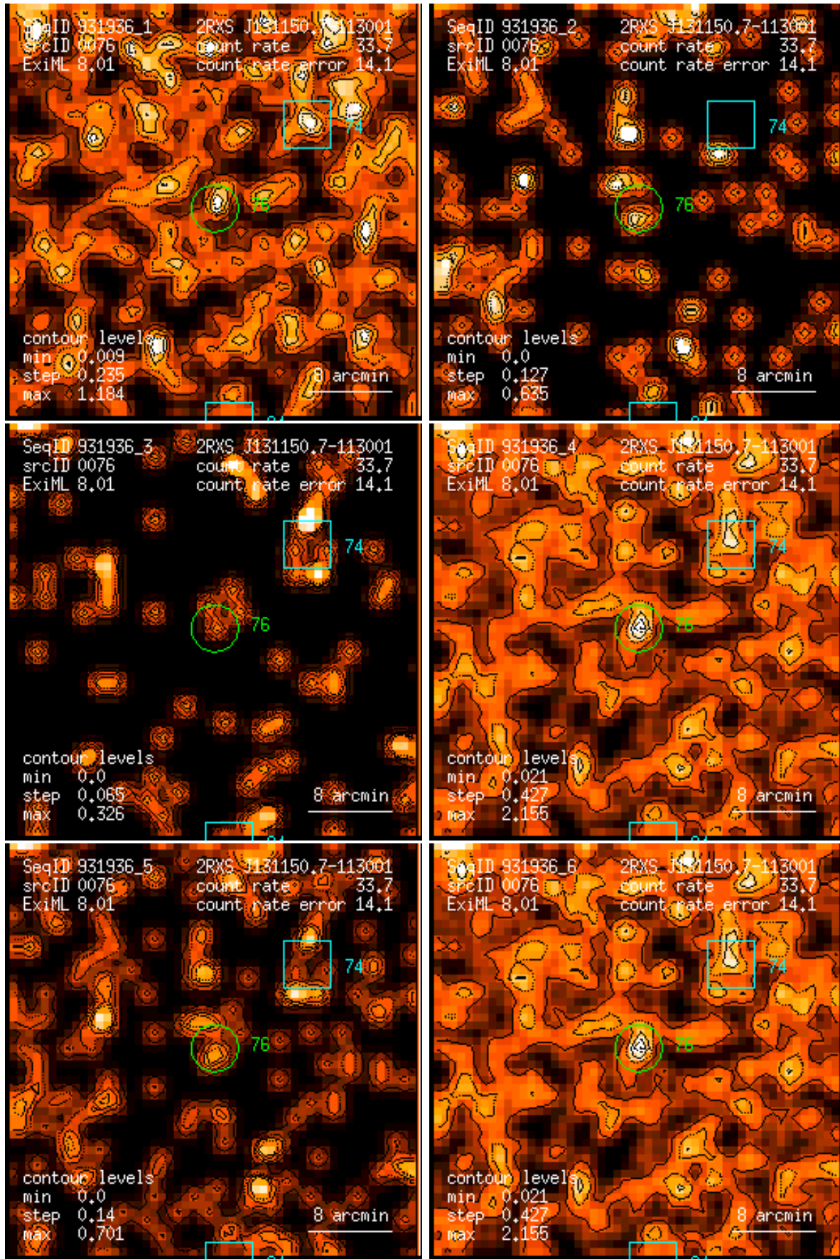
Figure 76: RASS 931936: detection 0076: band rate images, Gaussian filter: (1) PSPC channels 11 – 41, (2) 52 – 90, (3) 91 – 201, (4) 11 – 235, (5) 52 – 201, (6) 11 – 201. Broad band rates in counts/ks. Band rate contour levels in counts/ks/arcmin 2 .
