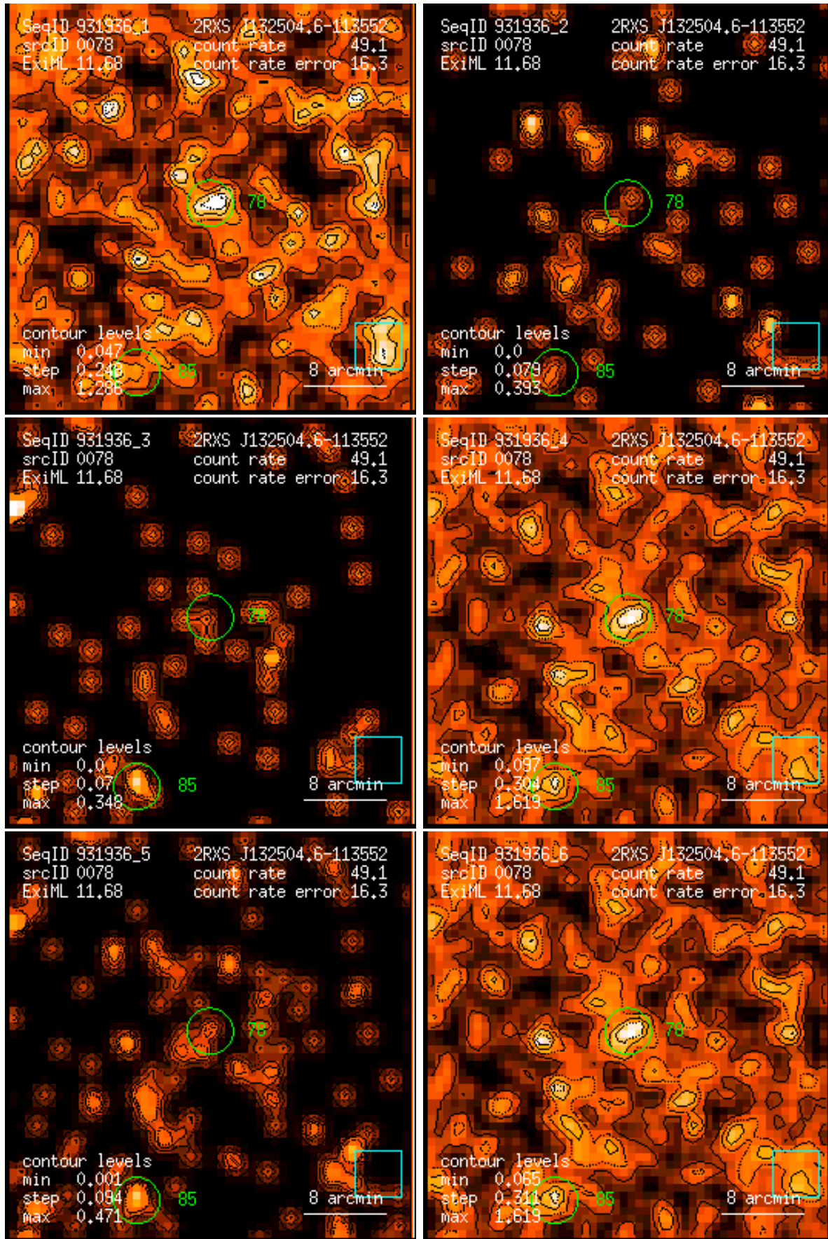
Figure 78: RASS 931936: detection 0078: band rate images, Gaussian filter: (1) PSPC channels 11 – 41, (2) 52 – 90, (3) 91 – 201, (4) 11 – 235, (5) 52 – 201, (6) 11 – 201. Broad band rates in counts/ks. Band rate contour levels in counts/ks/arcmin 2 .
