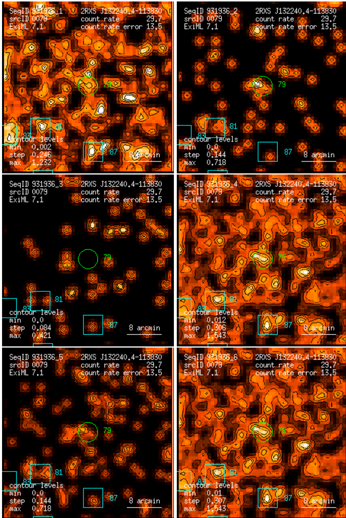
Figure 79: RASS 931936: detection 0079: band rate images, Gaussian filter: (1) PSPC channels 11 – 41, (2) 52 – 90, (3) 91 – 201, (4) 11 – 235, (5) 52 – 201, (6) 11 – 201. Broad band rates in counts/ks. Band rate contour levels in counts/ks/arcmin 2 .
