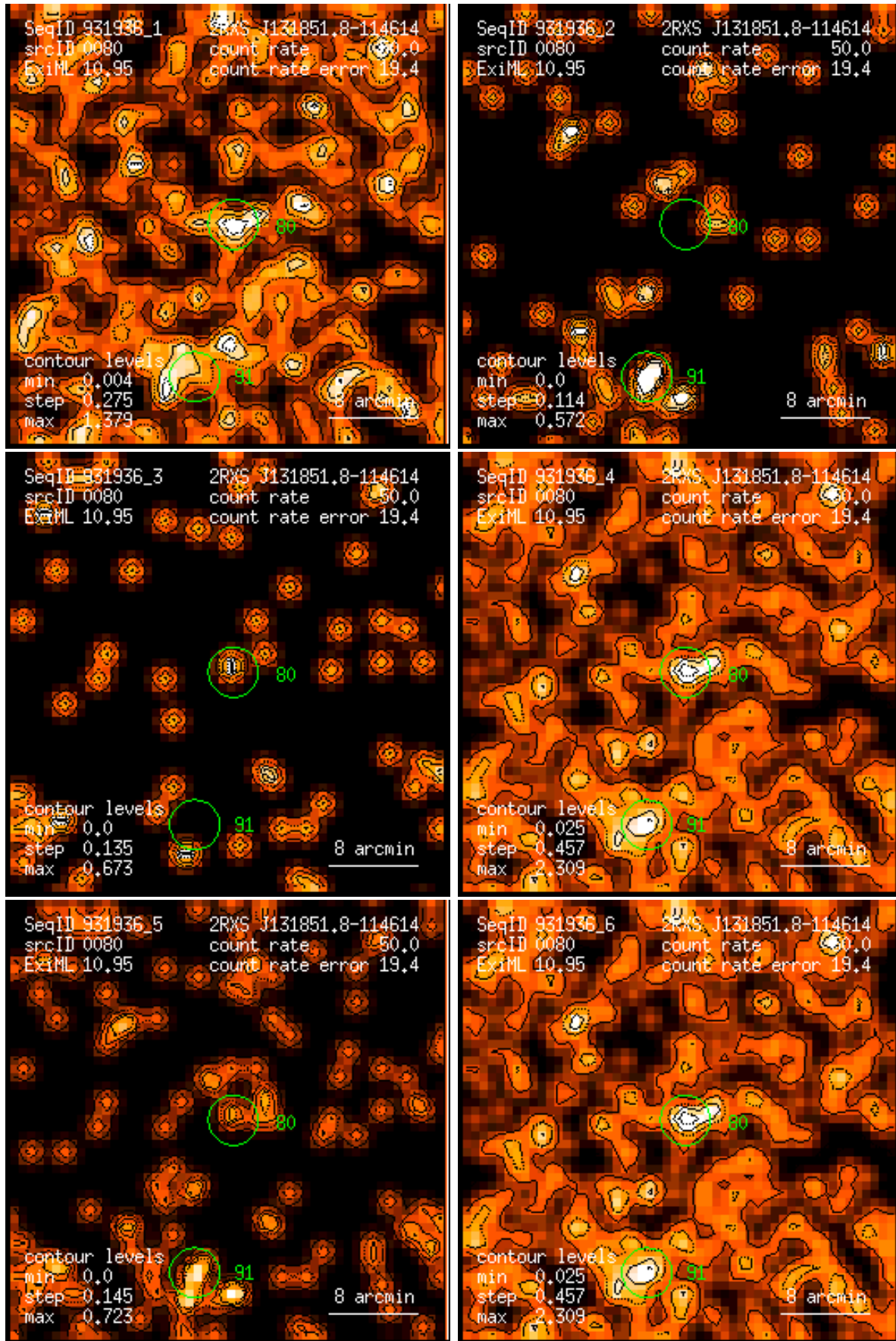
Figure 80: RASS 931936: detection 0080: band rate images, Gaussian filter: (1) PSPC channels 11 – 41, (2) 52 – 90, (3) 91 – 201, (4) 11 – 235, (5) 52 – 201, (6) 11 – 201. Broad band rates in counts/ks. Band rate contour levels in counts/ks/arcmin 2 .
