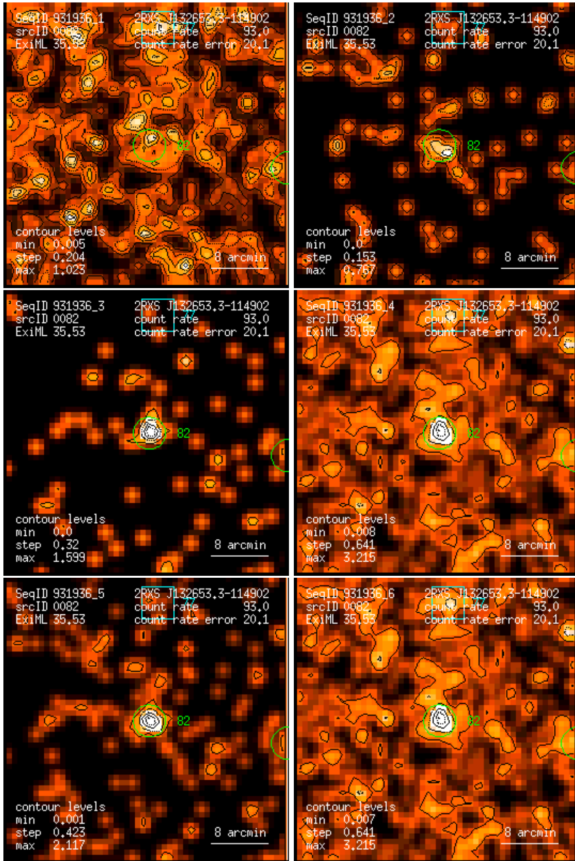
Figure 82: RASS 931936: detection 0082: band rate images, Gaussian filter: (1) PSPC channels 11 – 41, (2) 52 – 90, (3) 91 – 201, (4) 11 – 235, (5) 52 – 201, (6) 11 – 201. Broad band rates in counts/ks. Band rate contour levels in counts/ks/arcmin 2 .
