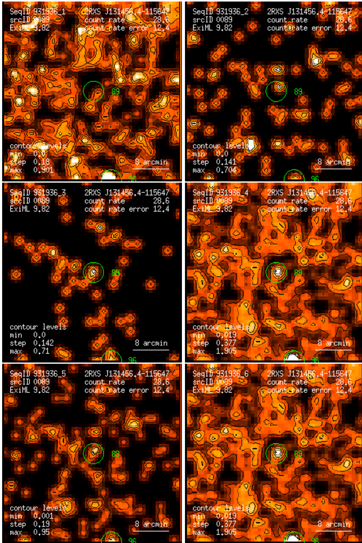
Figure 89: RASS 931936: detection 0089: band rate images, Gaussian filter: (1) PSPC channels 11 – 41, (2) 52 – 90, (3) 91 – 201, (4) 11 – 235, (5) 52 – 201, (6) 11 – 201. Broad band rates in counts/ks. Band rate contour levels in counts/ks/arcmin 2 .
