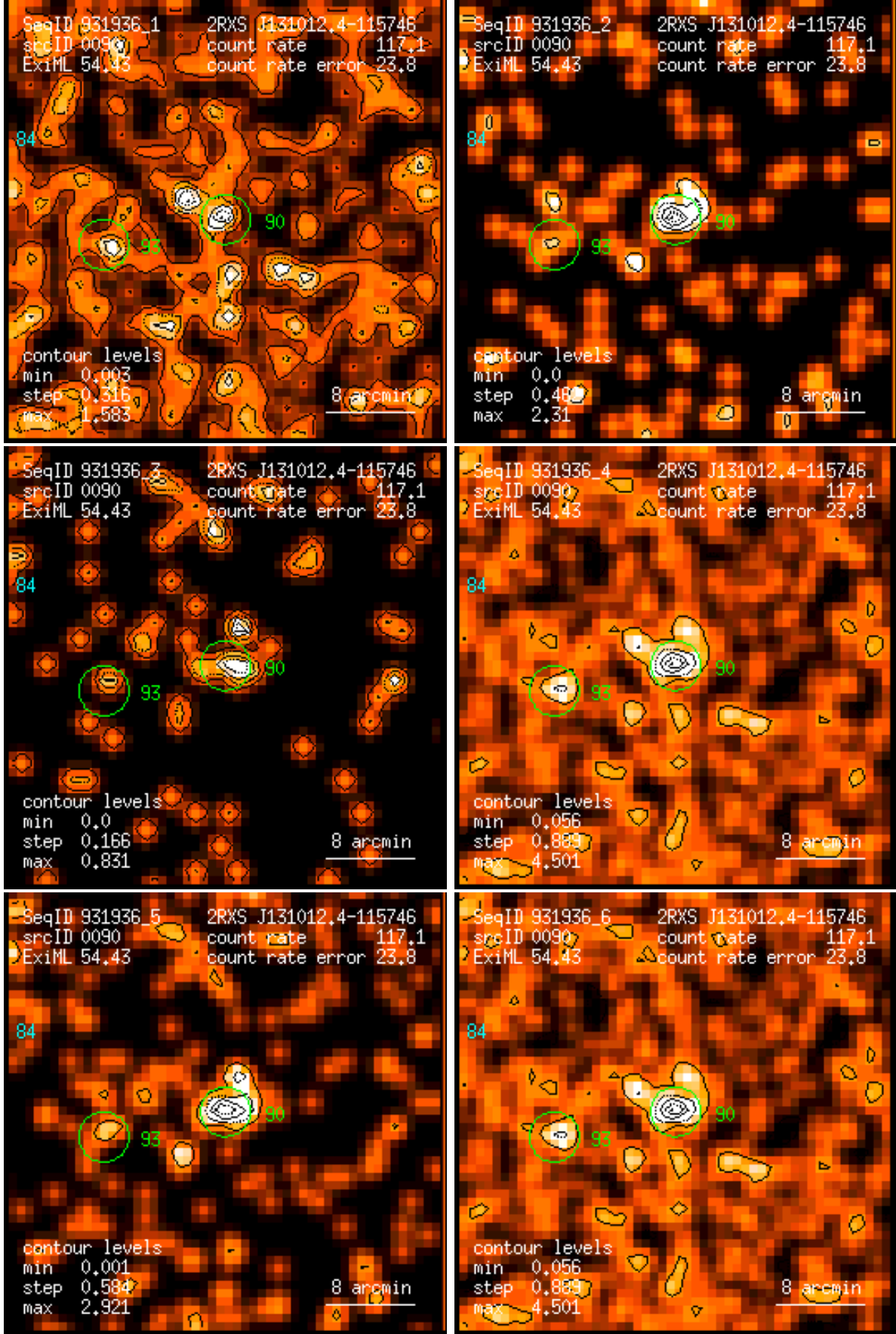
Figure 90: RASS 931936: detection 0090: band rate images, Gaussian filter: (1) PSPC channels 11 – 41, (2) 52 – 90, (3) 91 – 201, (4) 11 – 235, (5) 52 – 201, (6) 11 – 201. Broad band rates in counts/ks. Band rate contour levels in counts/ks/arcmin 2 .
