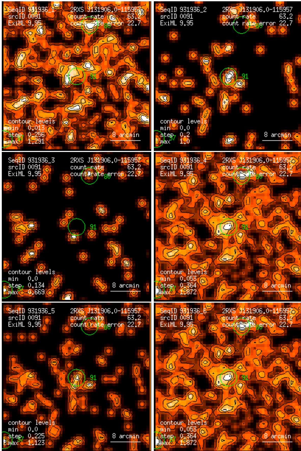
Figure 91: RASS 931936: detection 0091: band rate images, Gaussian filter: (1) PSPC channels 11 – 41, (2) 52 – 90, (3) 91 – 201, (4) 11 – 235, (5) 52 – 201, (6) 11 – 201. Broad band rates in counts/ks. Band rate contour levels in counts/ks/arcmin 2 .
