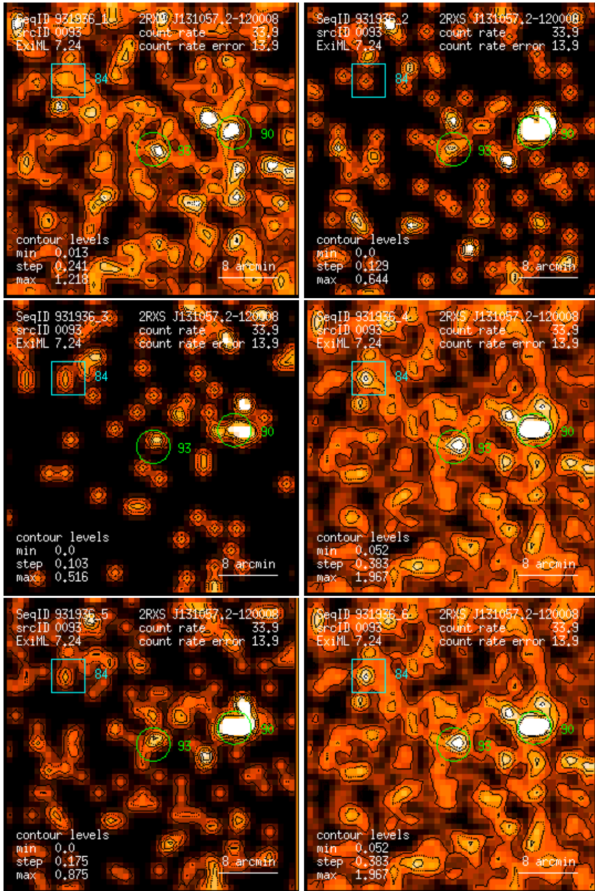
Figure 93: RASS 931936: detection 0093: band rate images, Gaussian filter: (1) PSPC channels 11 – 41, (2) 52 – 90, (3) 91 – 201, (4) 11 – 235, (5) 52 – 201, (6) 11 – 201. Broad band rates in counts/ks. Band rate contour levels in counts/ks/arcmin 2 .
