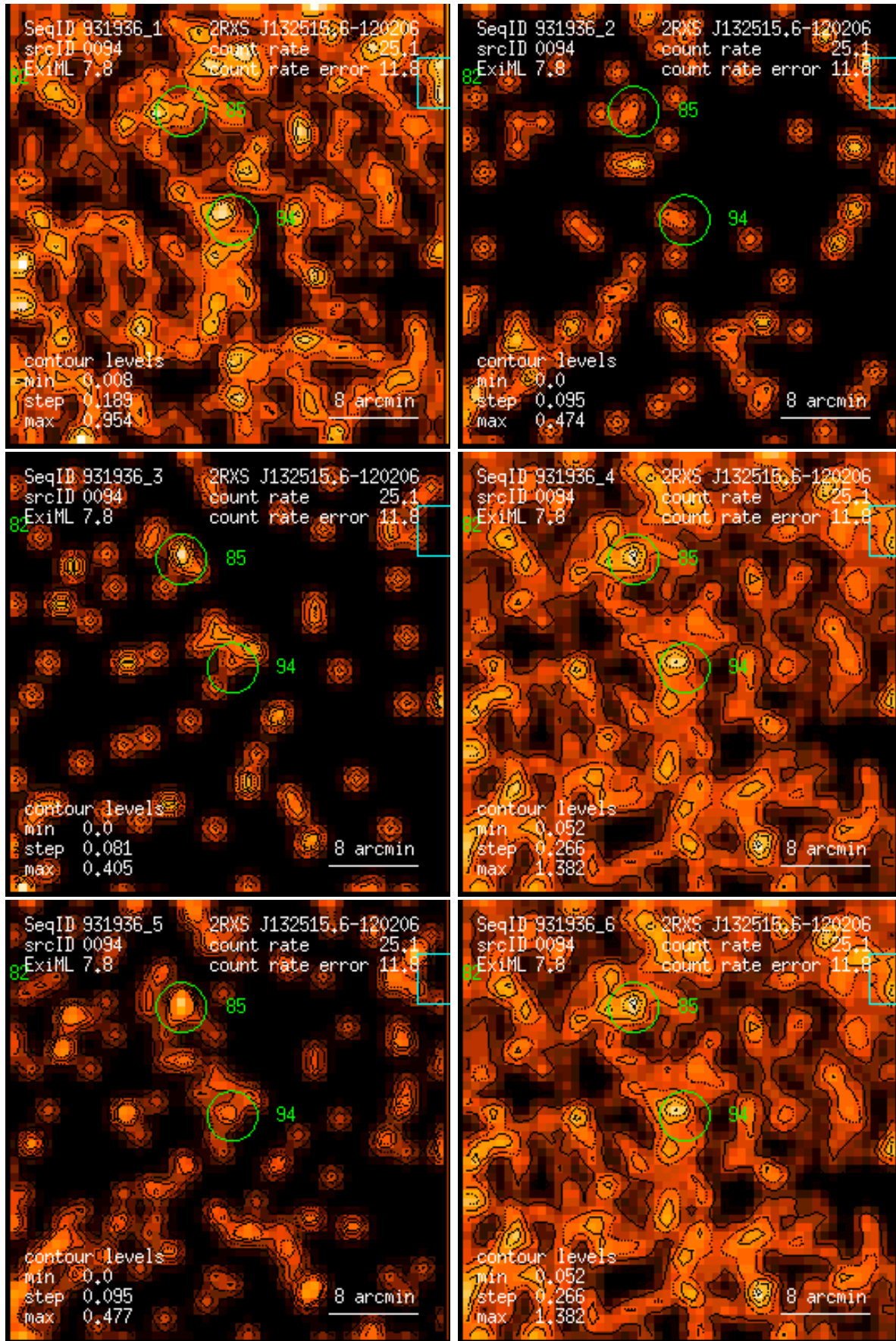
Figure 94: RASS 931936: detection 0094: band rate images, Gaussian filter: (1) PSPC channels 11 – 41, (2) 52 – 90, (3) 91 – 201, (4) 11 – 235, (5) 52 – 201, (6) 11 – 201. Broad band rates in counts/ks. Band rate contour levels in counts/ks/arcmin 2 .
