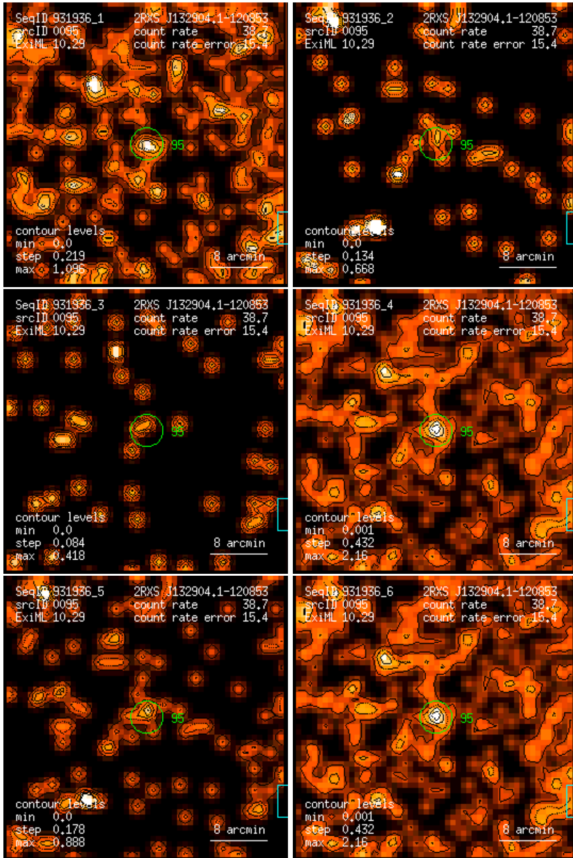
Figure 95: RASS 931936: detection 0095: band rate images, Gaussian filter: (1) PSPC channels 11 – 41, (2) 52 – 90, (3) 91 – 201, (4) 11 – 235, (5) 52 – 201, (6) 11 – 201. Broad band rates in counts/ks. Band rate contour levels in counts/ks/arcmin 2 .
