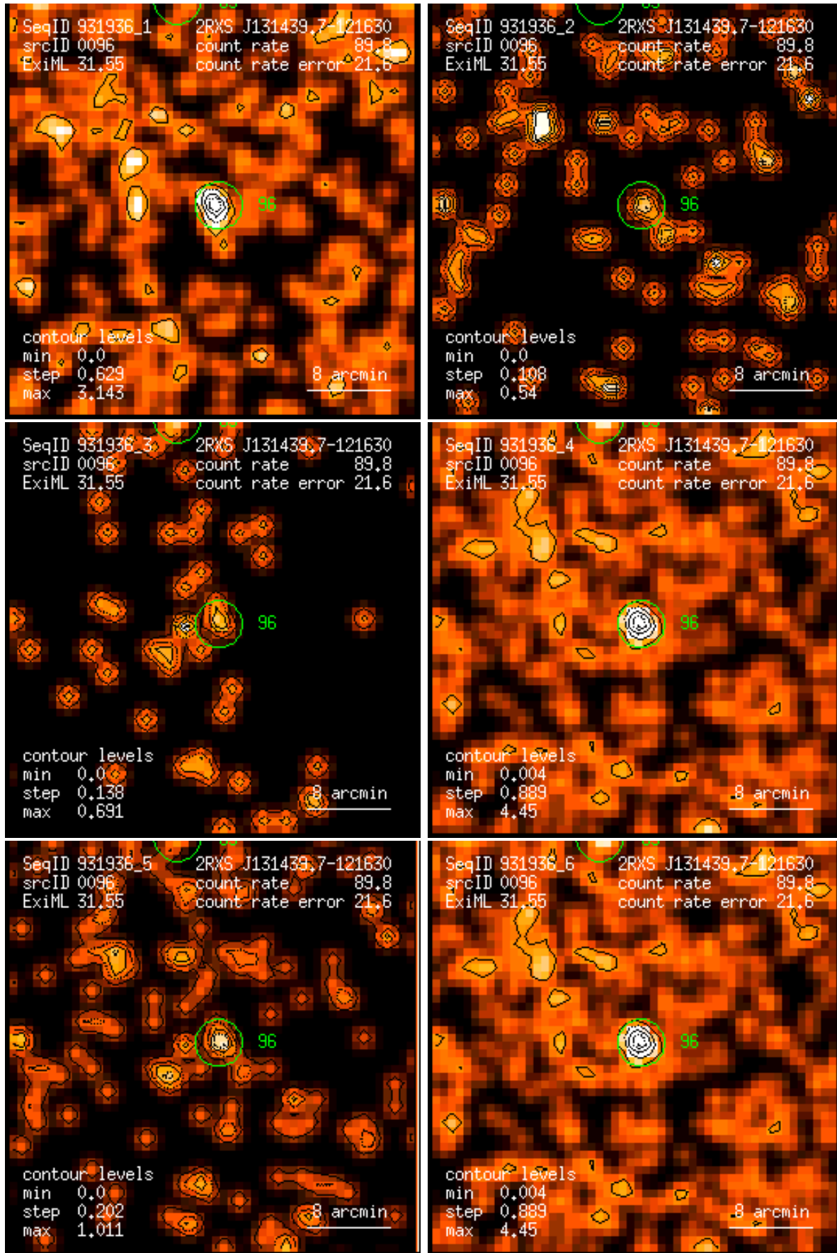
Figure 96: RASS 931936: detection 0096: band rate images, Gaussian filter: (1) PSPC channels 11 – 41, (2) 52 – 90, (3) 91 – 201, (4) 11 – 235, (5) 52 – 201, (6) 11 – 201. Broad band rates in counts/ks. Band rate contour levels in counts/ks/arcmin 2 .
