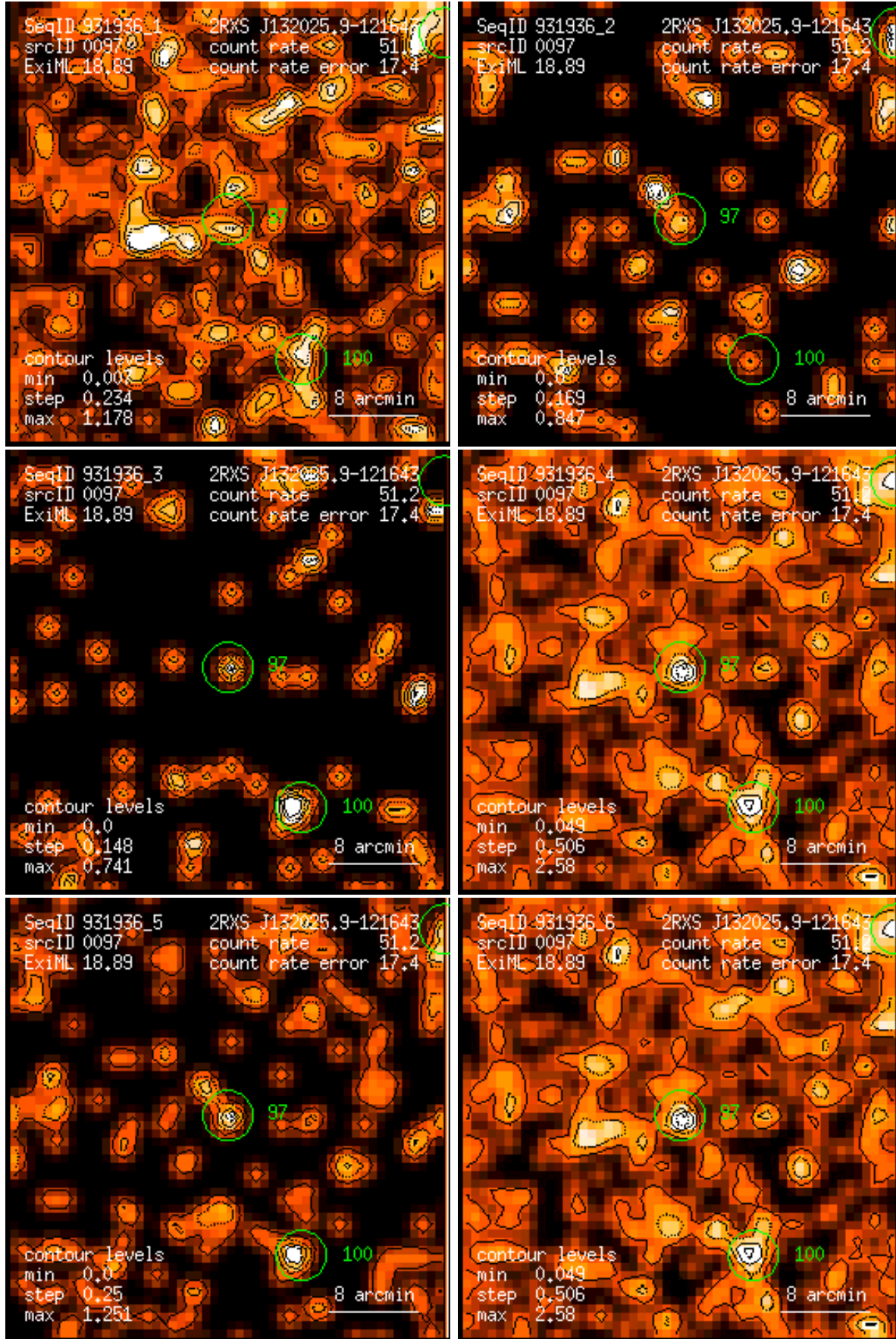
Figure 97: RASS 931936: detection 0097: band rate images, Gaussian filter: (1) PSPC channels 11 – 41, (2) 52 – 90, (3) 91 – 201, (4) 11 – 235, (5) 52 – 201, (6) 11 – 201. Broad band rates in counts/ks. Band rate contour levels in counts/ks/arcmin 2 .
