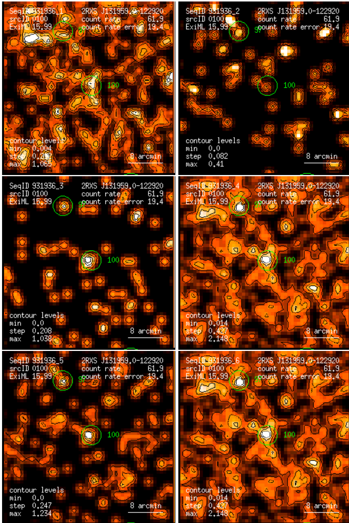
Figure 100: RASS 931936: detection 0100: band rate images, Gaussian filter: (1) PSPC channels 11 – 41, (2) 52 – 90, (3) 91 – 201, (4) 11 – 235, (5) 52 – 201, (6) 11 – 201. Broad band rates in counts/ks. Band rate contour levels in counts/ks/arcmin 2 .
