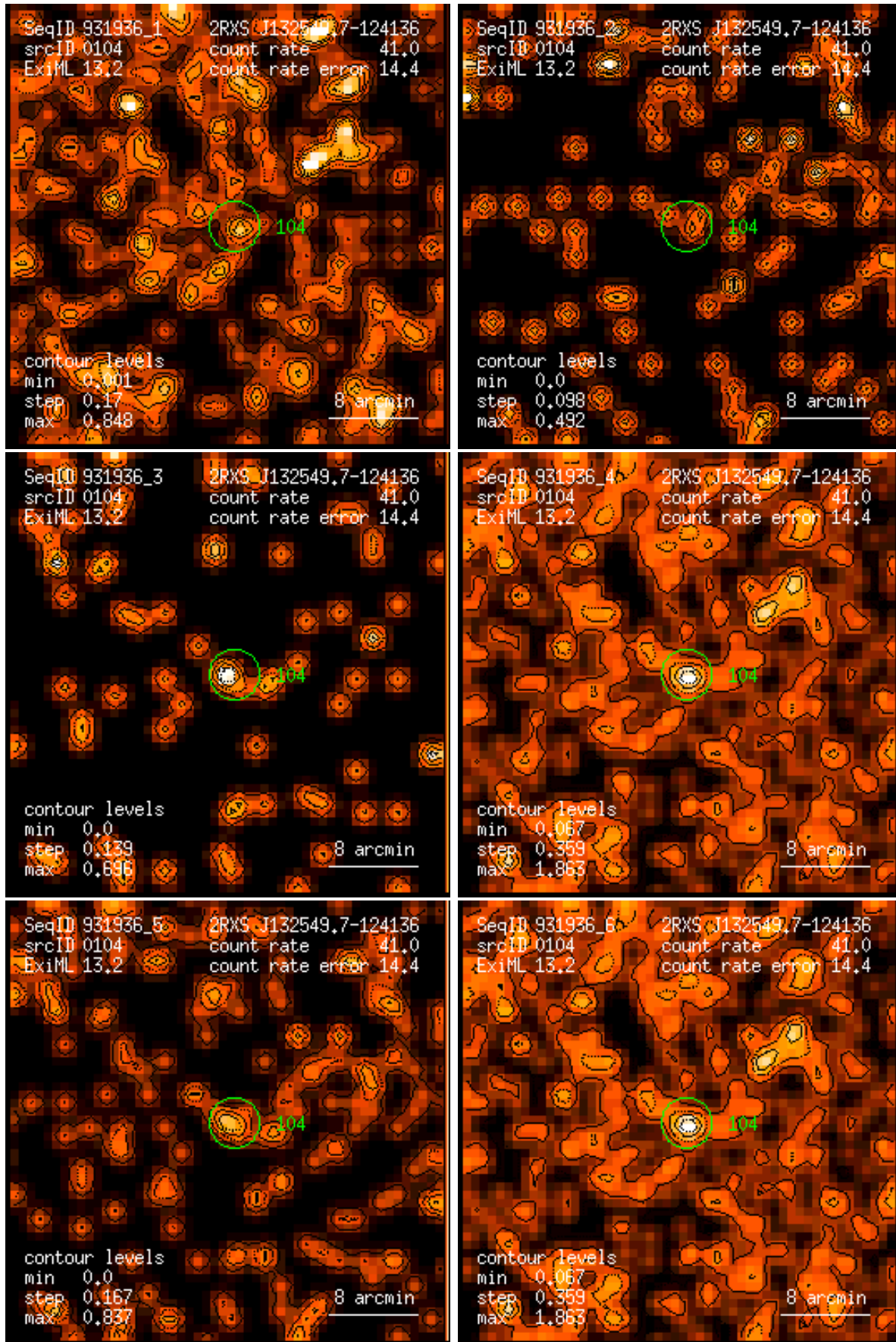
Figure 104: RASS 931936: detection 0104: band rate images, Gaussian filter: (1) PSPC channels 11 – 41, (2) 52 – 90, (3) 91 – 201, (4) 11 – 235, (5) 52 – 201, (6) 11 – 201. Broad band rates in counts/ks. Band rate contour levels in counts/ks/arcmin 2 .
