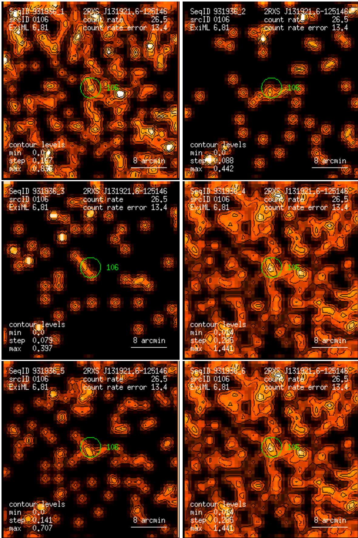
Figure 106: RASS 931936: detection 0106: band rate images, Gaussian filter: (1) PSPC channels 11 – 41, (2) 52 – 90, (3) 91 – 201, (4) 11 – 235, (5) 52 – 201, (6) 11 – 201. Broad band rates in counts/ks. Band rate contour levels in counts/ks/arcmin 2 .
