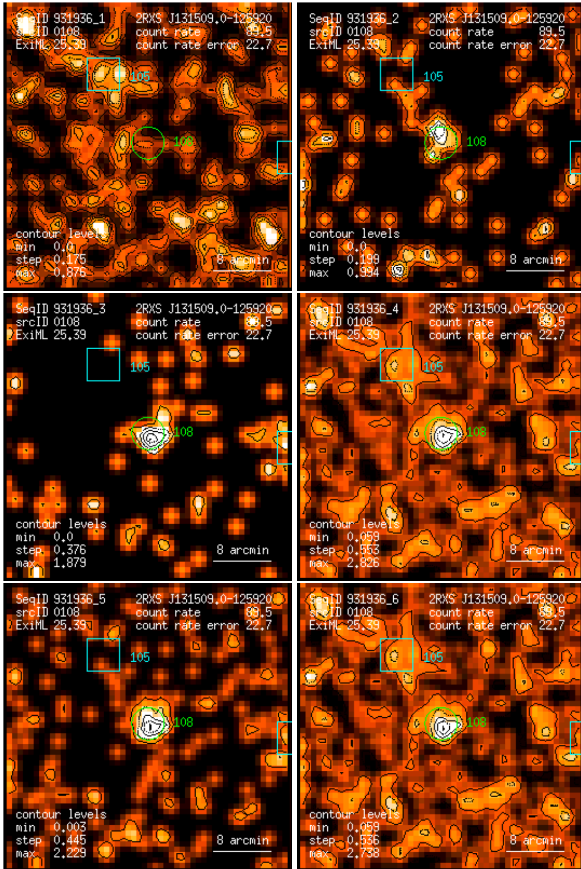
Figure 108: RASS 931936: detection 0108: band rate images, Gaussian filter: (1) PSPC channels 11 – 41, (2) 52 – 90, (3) 91 – 201, (4) 11 – 235, (5) 52 – 201, (6) 11 – 201. Broad band rates in counts/ks. Band rate contour levels in counts/ks/arcmin 2 .
