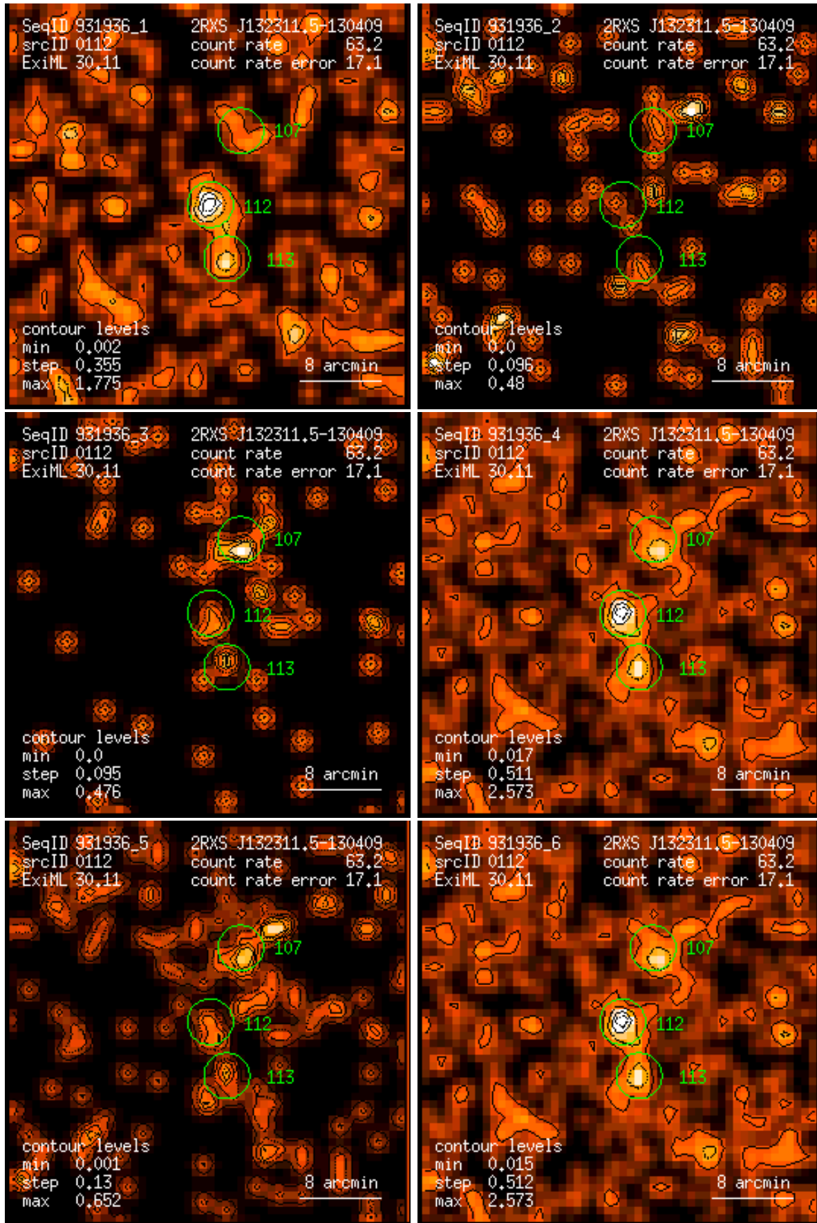
Figure 112: RASS 931936: detection 0112: band rate images, Gaussian filter: (1) PSPC channels 11 – 41, (2) 52 – 90, (3) 91 – 201, (4) 11 – 235, (5) 52 – 201, (6) 11 – 201. Broad band rates in counts/ks. Band rate contour levels in counts/ks/arcmin 2 .
