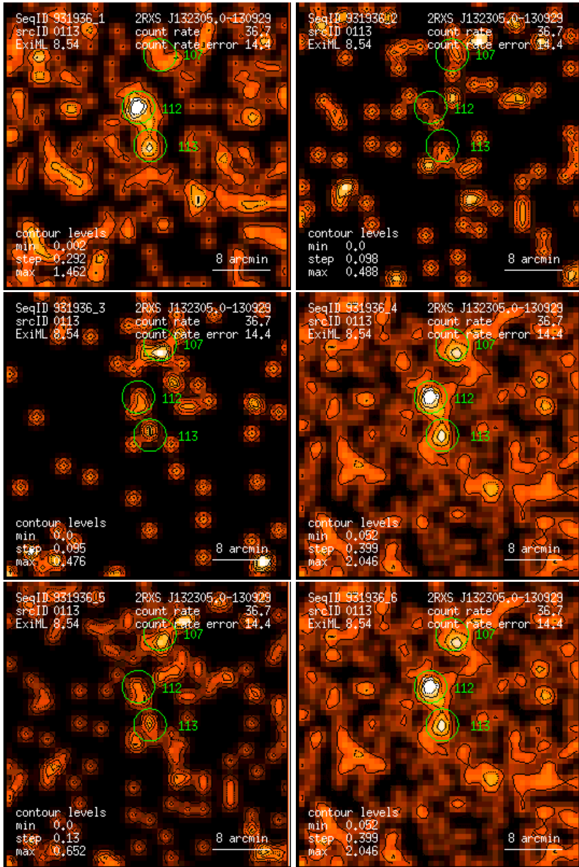
Figure 113: RASS 931936: detection 0113: band rate images, Gaussian filter: (1) PSPC channels 11 – 41, (2) 52 – 90, (3) 91 – 201, (4) 11 – 235, (5) 52 – 201, (6) 11 – 201. Broad band rates in counts/ks. Band rate contour levels in counts/ks/arcmin 2 .
