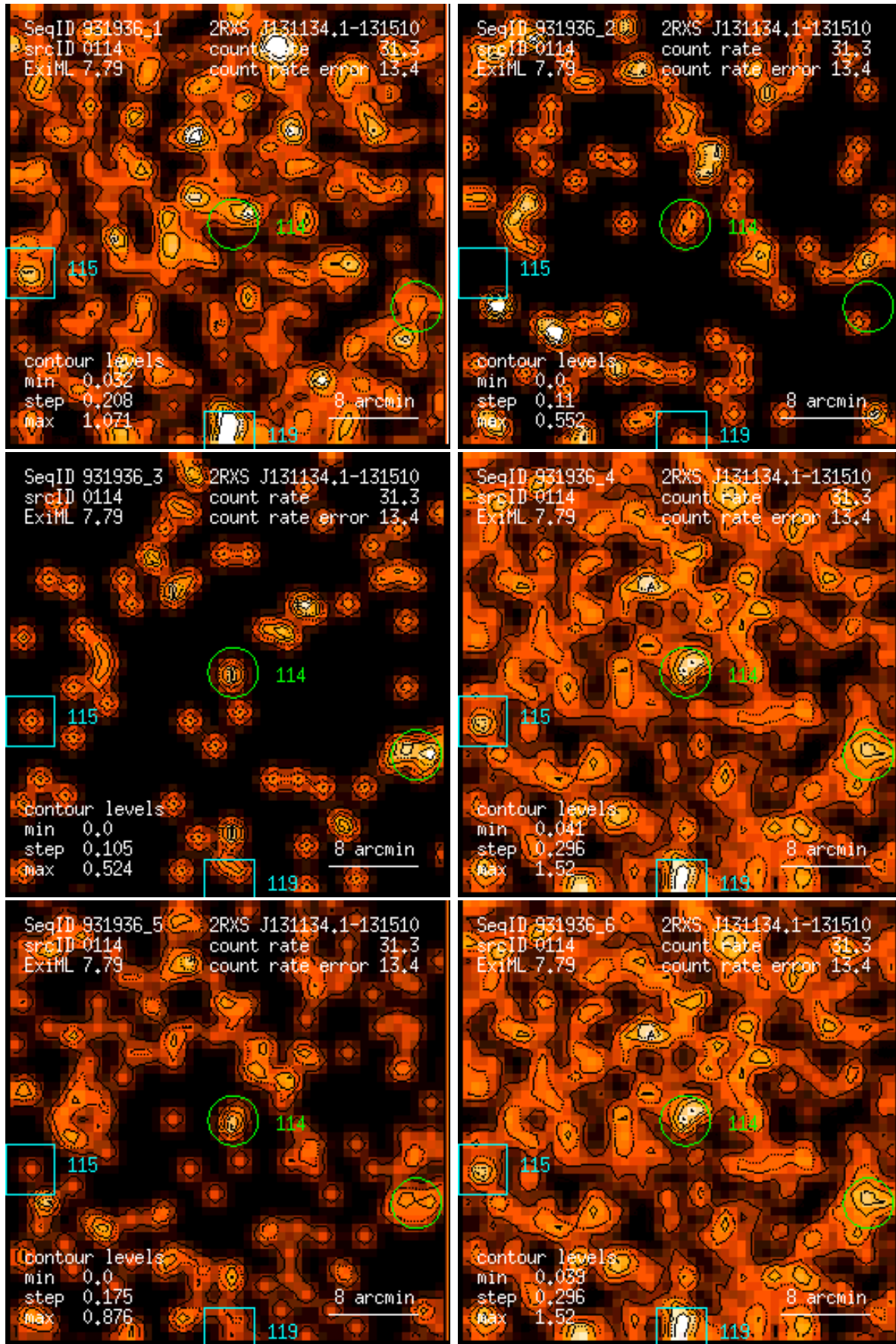
Figure 114: RASS 931936: detection 0114: band rate images, Gaussian filter: (1) PSPC channels 11 – 41, (2) 52 – 90, (3) 91 – 201, (4) 11 – 235, (5) 52 – 201, (6) 11 – 201. Broad band rates in counts/ks. Band rate contour levels in counts/ks/arcmin 2 .
