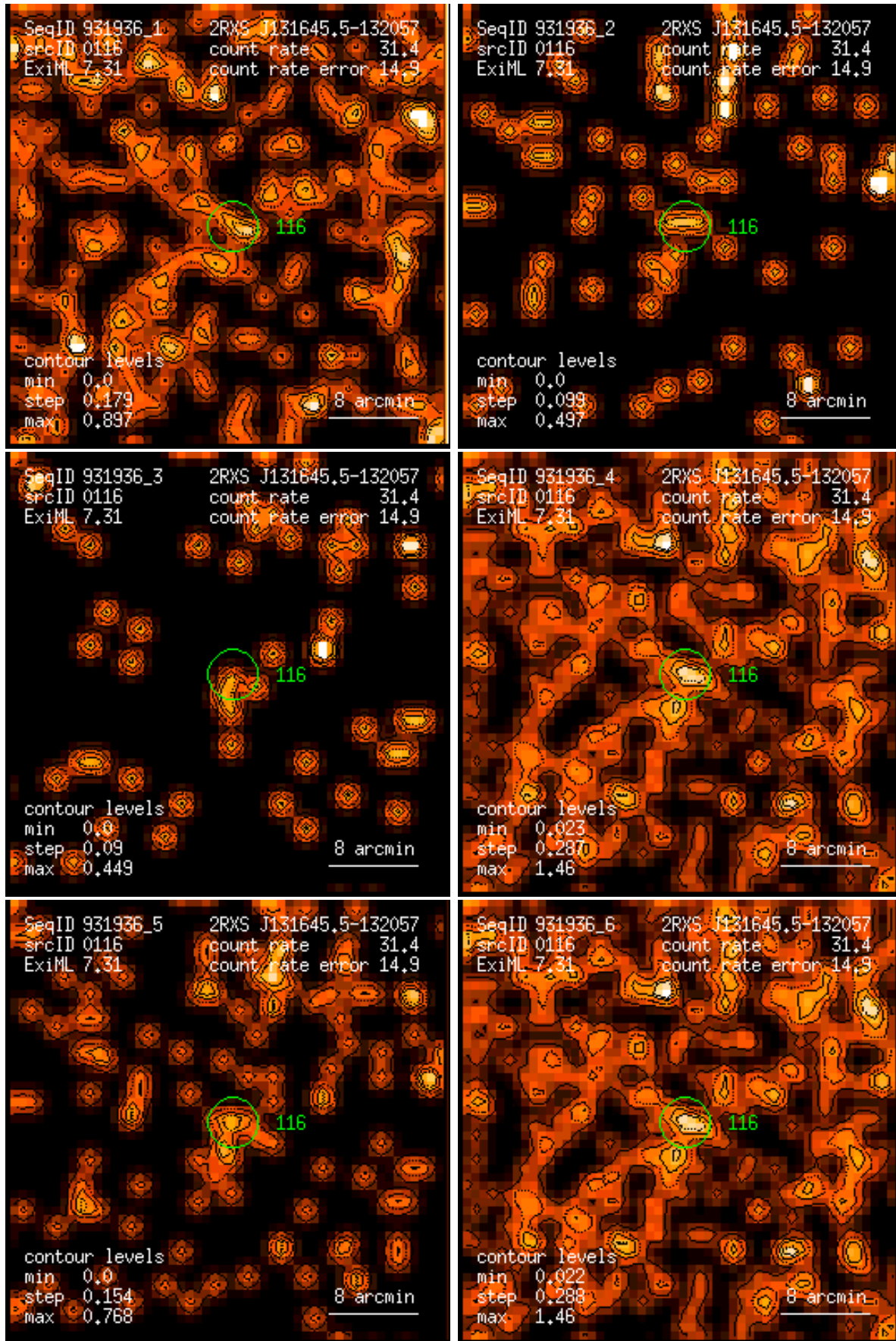
Figure 116: RASS 931936: detection 0116: band rate images, Gaussian filter: (1) PSPC channels 11 – 41, (2) 52 – 90, (3) 91 – 201, (4) 11 – 235, (5) 52 – 201, (6) 11 – 201. Broad band rates in counts/ks. Band rate contour levels in counts/ks/arcmin 2 .
