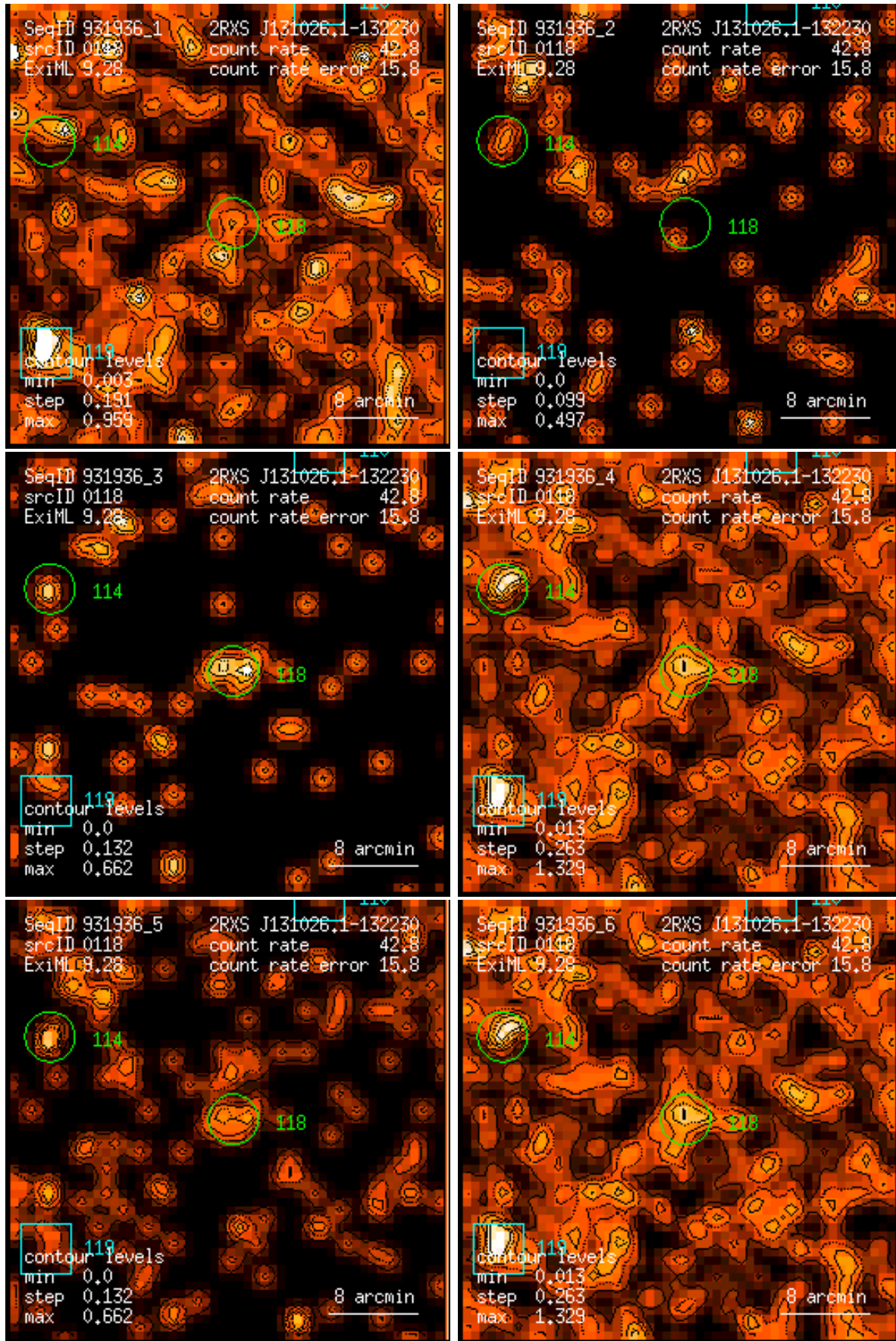
Figure 118: RASS 931936: detection 0118: band rate images, Gaussian filter: (1) PSPC channels 11 – 41, (2) 52 – 90, (3) 91 – 201, (4) 11 – 235, (5) 52 – 201, (6) 11 – 201. Broad band rates in counts/ks. Band rate contour levels in counts/ks/arcmin 2 .
