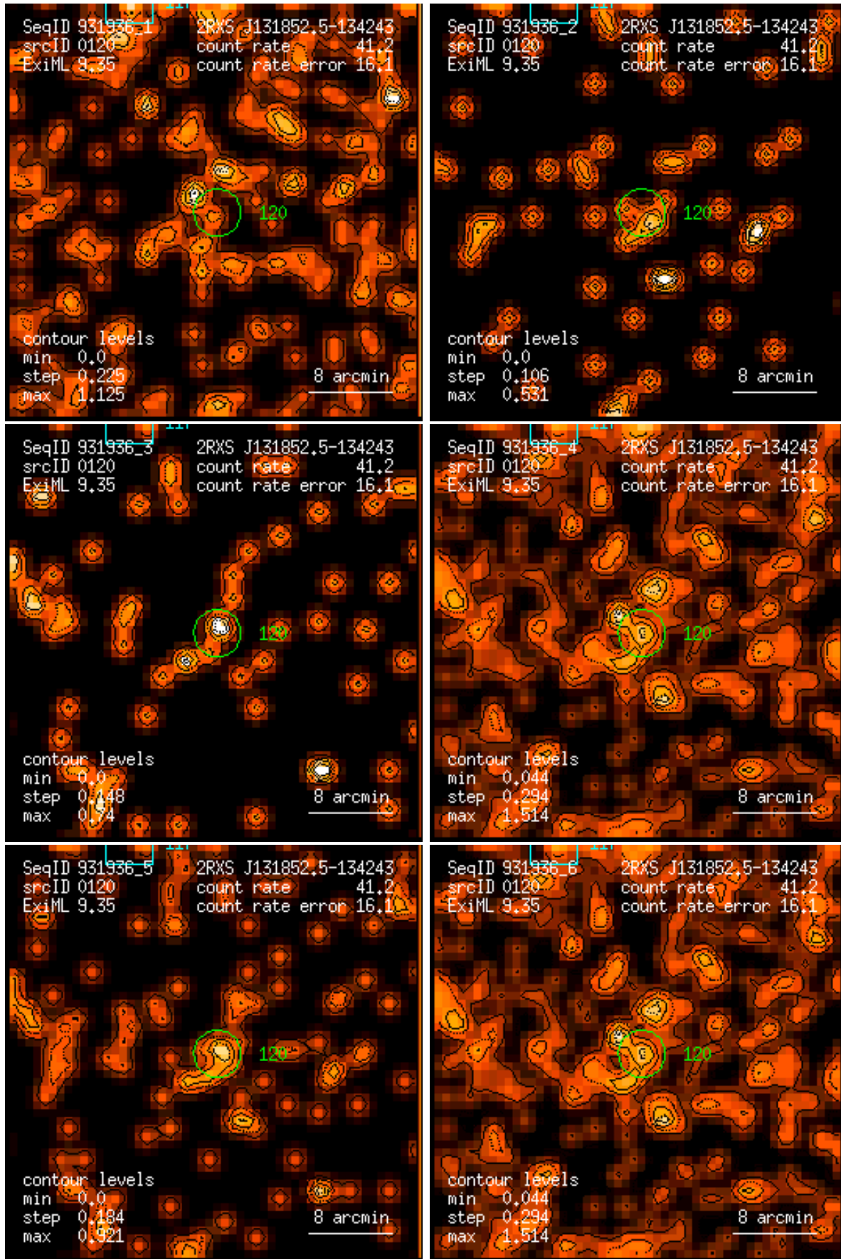
Figure 120: RASS 931936: detection 0120: band rate images, Gaussian filter: (1) PSPC channels 11 – 41, (2) 52 – 90, (3) 91 – 201, (4) 11 – 235, (5) 52 – 201, (6) 11 – 201. Broad band rates in counts/ks. Band rate contour levels in counts/ks/arcmin 2 .
