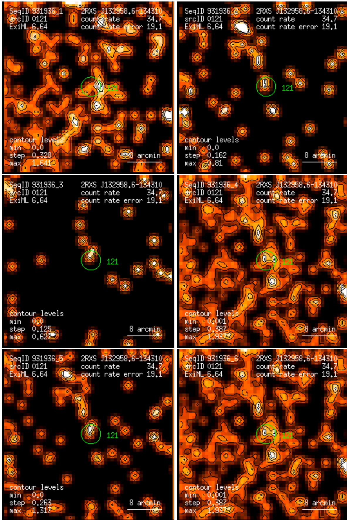
Figure 121: RASS 931936: detection 0121: band rate images, Gaussian filter: (1) PSPC channels 11 – 41, (2) 52 – 90, (3) 91 – 201, (4) 11 – 235, (5) 52 – 201, (6) 11 – 201. Broad band rates in counts/ks. Band rate contour levels in counts/ks/arcmin 2 .
