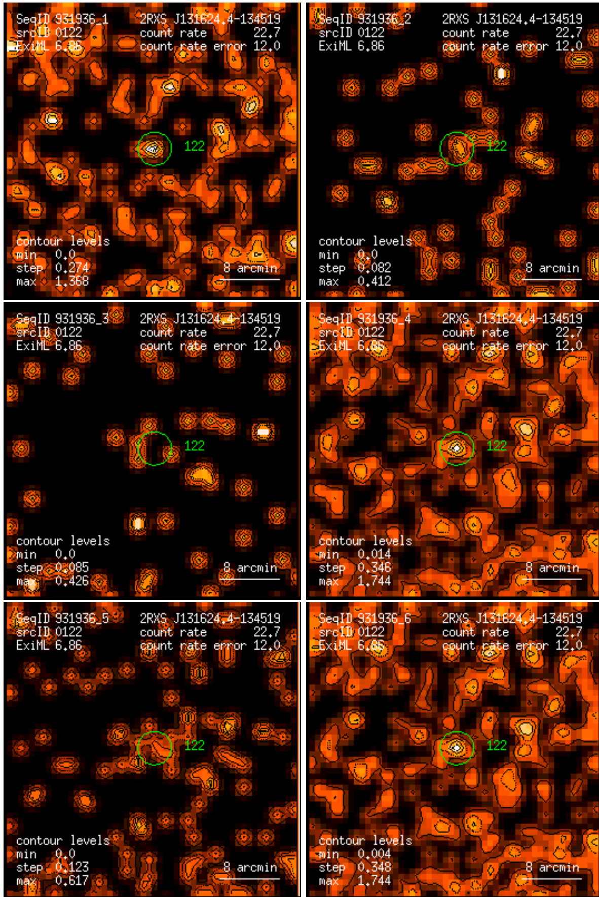
Figure 122: RASS 931936: detection 0122: band rate images, Gaussian filter: (1) PSPC channels 11 – 41, (2) 52 – 90, (3) 91 – 201, (4) 11 – 235, (5) 52 – 201, (6) 11 – 201. Broad band rates in counts/ks. Band rate contour levels in counts/ks/arcmin 2 .
