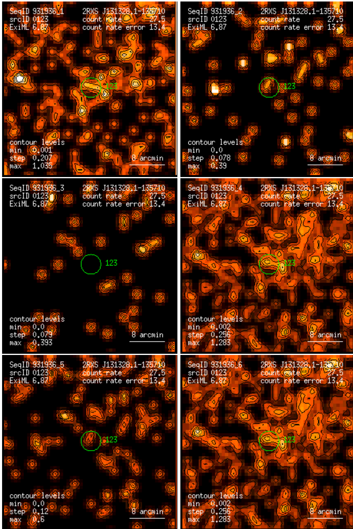
Figure 123: RASS 931936: detection 0123: band rate images, Gaussian filter: (1) PSPC channels 11 – 41, (2) 52 – 90, (3) 91 – 201, (4) 11 – 235, (5) 52 – 201, (6) 11 – 201. Broad band rates in counts/ks. Band rate contour levels in counts/ks/arcmin 2 .
