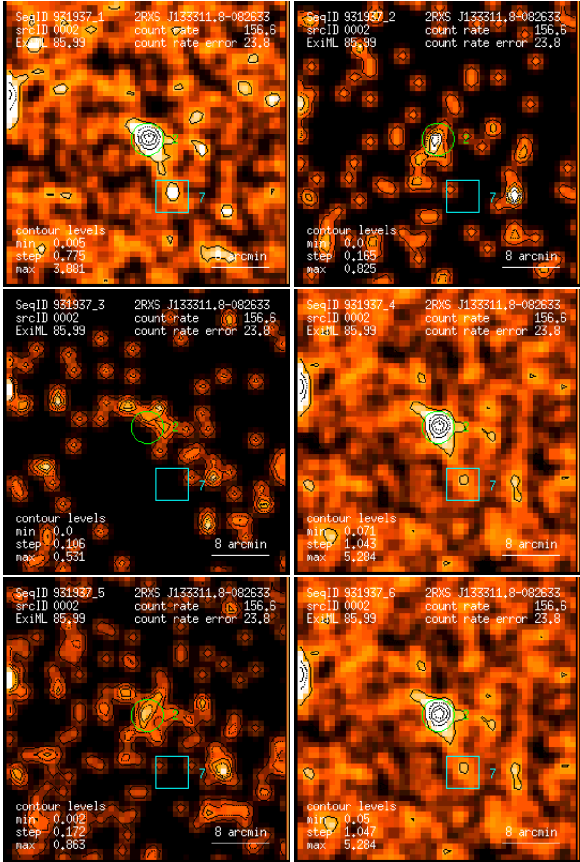
Figure 2: RASS 931937: detection 0002: band rate images, Gaussian filter: (1) PSPC channels 11 – 41, (2) 52 – 90, (3) 91 – 201, (4) 11 – 235, (5) 52 – 201, (6) 11 – 201. Broad band rates in counts/ks. Band rate contour levels in counts/ks/arcmin 2 .
