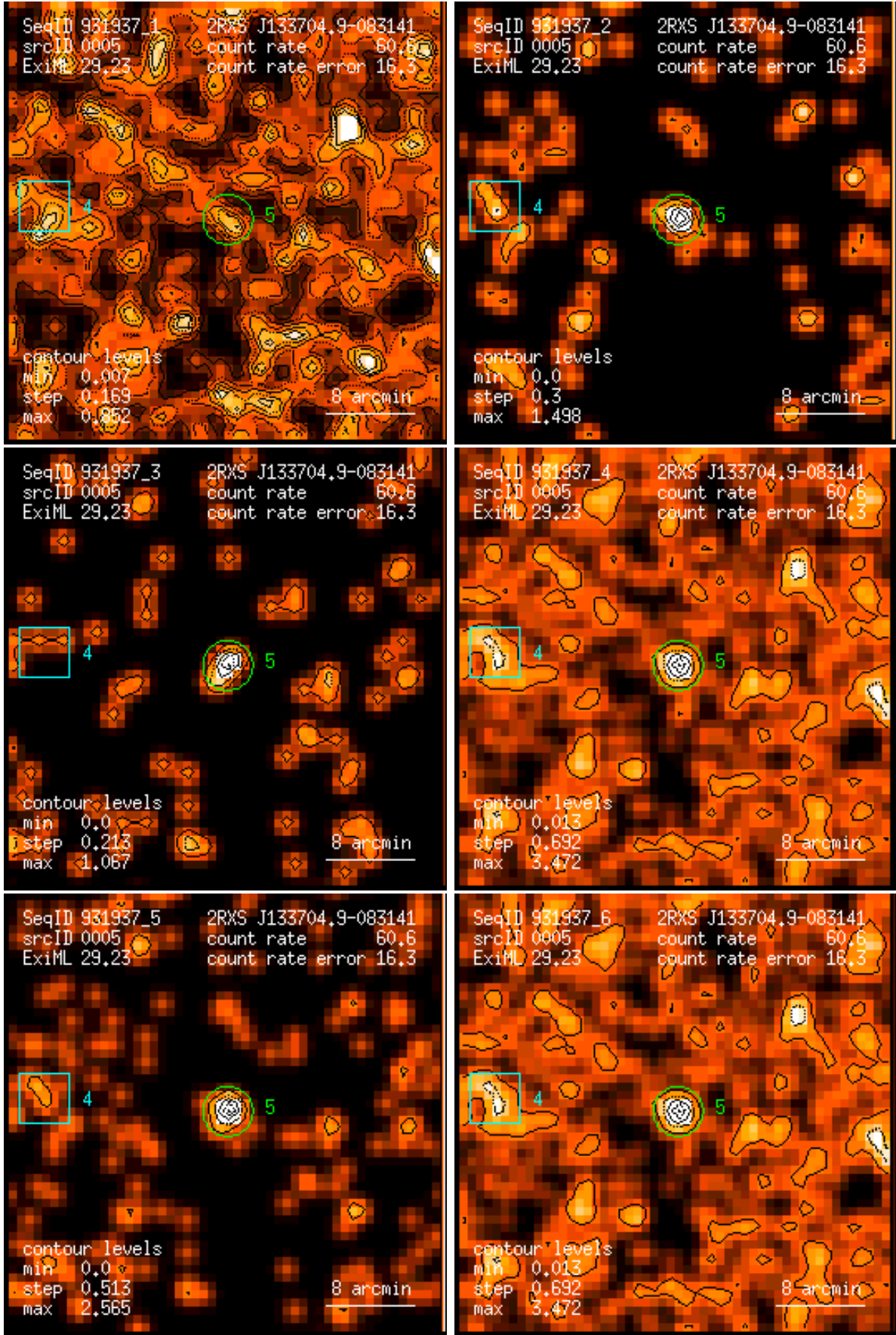
Figure 5: RASS 931937: detection 0005: band rate images, Gaussian filter: (1) PSPC channels 11 – 41, (2) 52 – 90, (3) 91 – 201, (4) 11 – 235, (5) 52 – 201, (6) 11 – 201. Broad band rates in counts/ks. Band rate contour levels in counts/ks/arcmin 2 .
