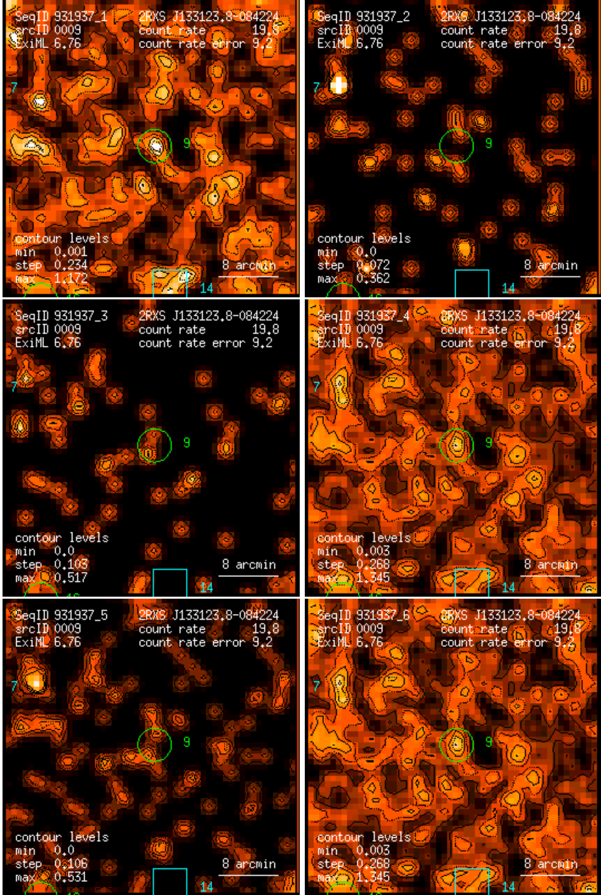
Figure 9: RASS 931937: detection 0009: band rate images, Gaussian filter: (1) PSPC channels 11 – 41, (2) 52 – 90, (3) 91 – 201, (4) 11 – 235, (5) 52 – 201, (6) 11 – 201. Broad band rates in counts/ks. Band rate contour levels in counts/ks/arcmin 2 .
