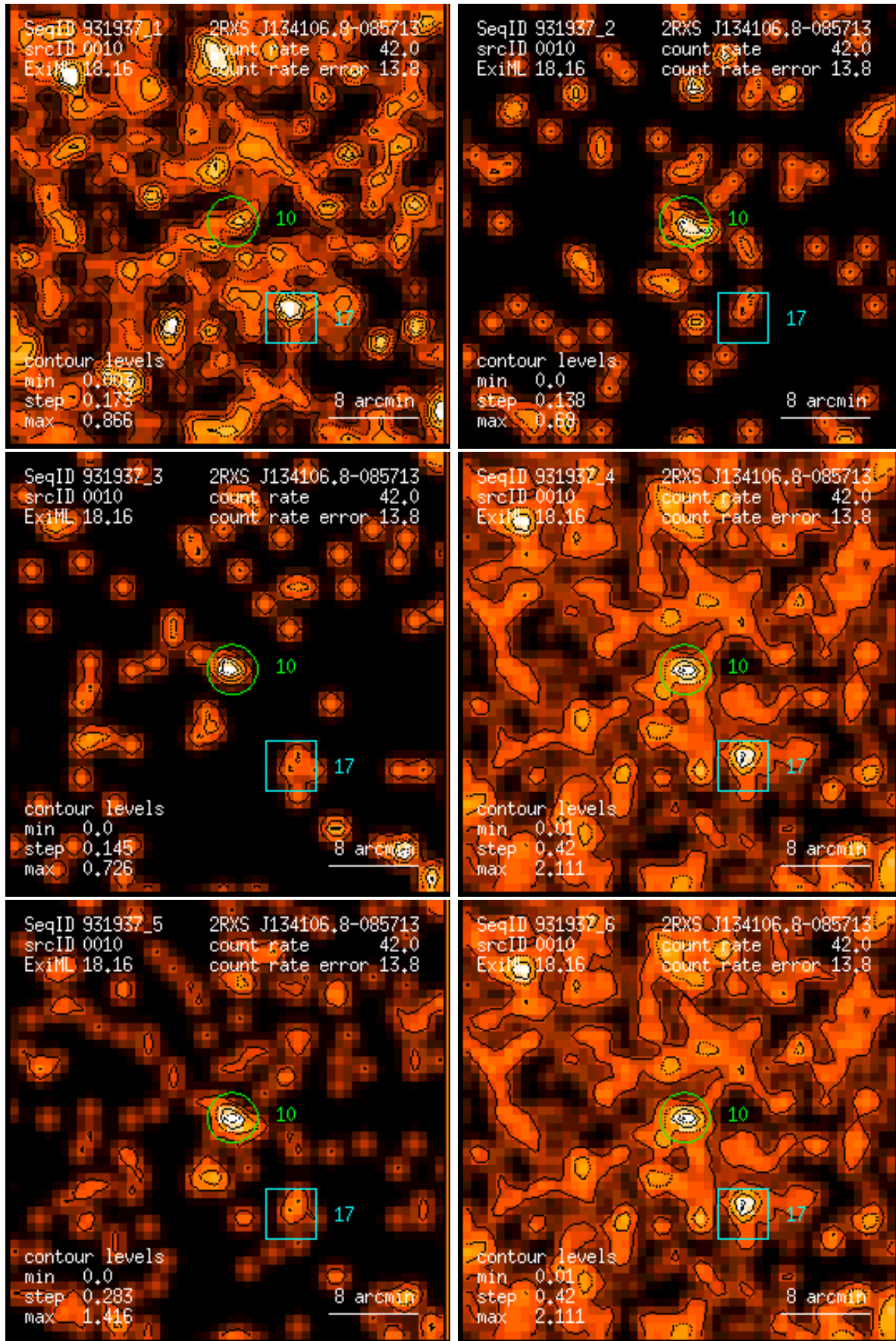
Figure 10: RASS 931937: detection 0010: band rate images, Gaussian filter: (1) PSPC channels 11 – 41, (2) 52 – 90, (3) 91 – 201, (4) 11 – 235, (5) 52 – 201, (6) 11 – 201. Broad band rates in counts/ks. Band rate contour levels in counts/ks/arcmin 2 .
