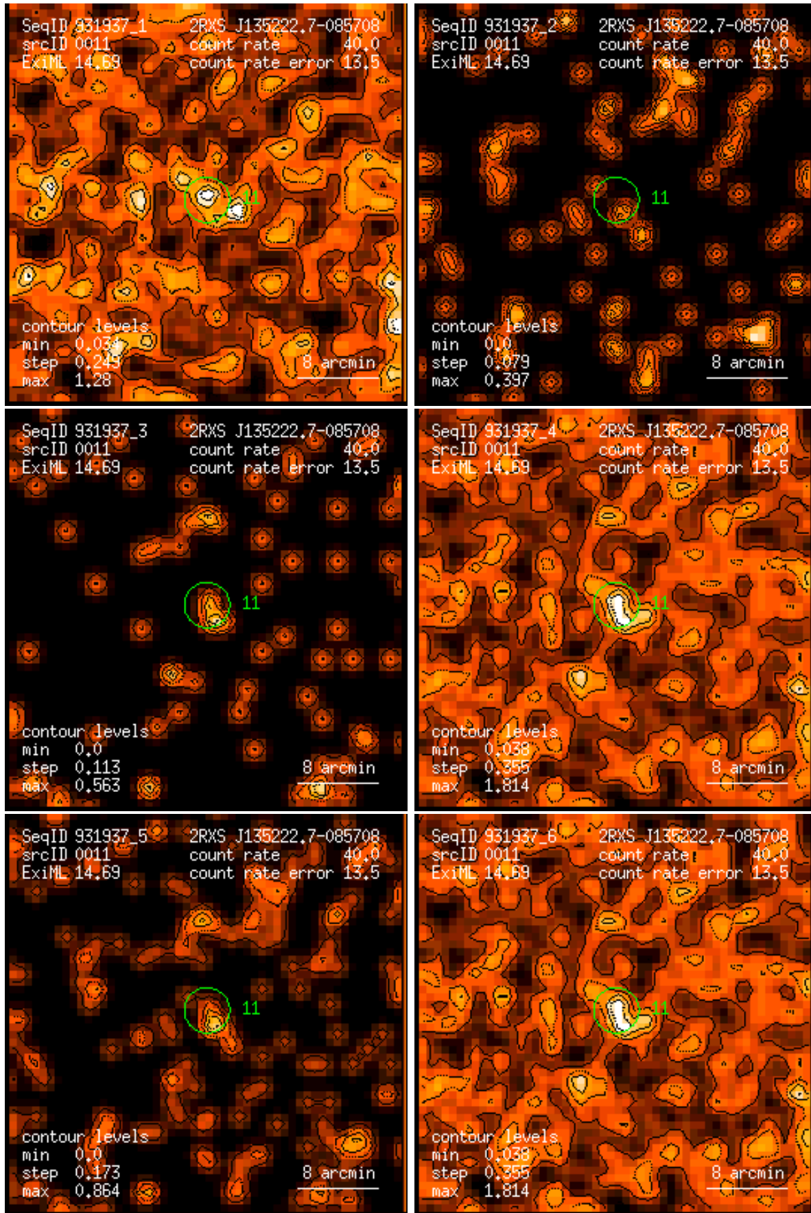
Figure 11: RASS 931937: detection 0011: band rate images, Gaussian filter: (1) PSPC channels 11 – 41, (2) 52 – 90, (3) 91 – 201, (4) 11 – 235, (5) 52 – 201, (6) 11 – 201. Broad band rates in counts/ks. Band rate contour levels in counts/ks/arcmin 2 .
