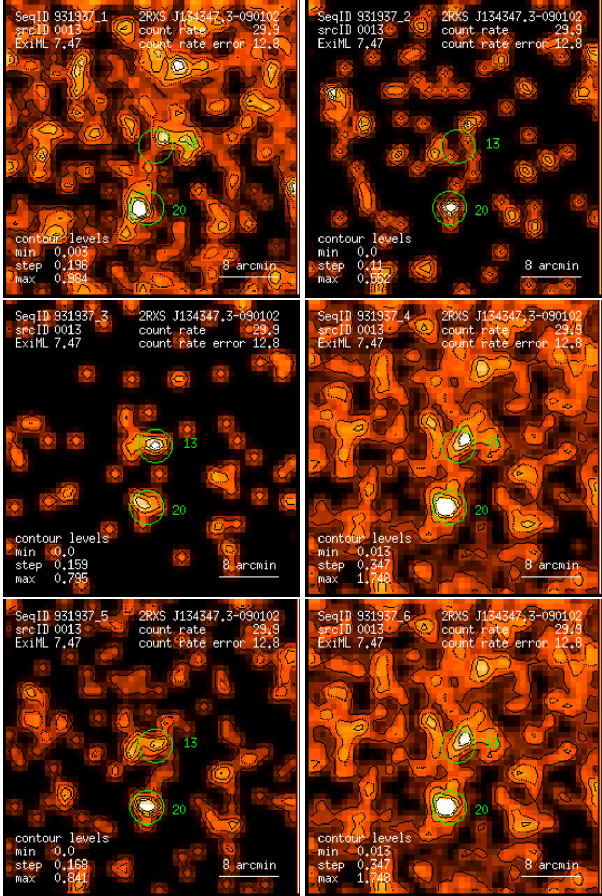
Figure 13: RASS 931937: detection 0013: band rate images, Gaussian filter: (1) PSPC channels 11 – 41, (2) 52 – 90, (3) 91 – 201, (4) 11 – 235, (5) 52 – 201, (6) 11 – 201. Broad band rates in counts/ks. Band rate contour levels in counts/ks/arcmin 2 .
