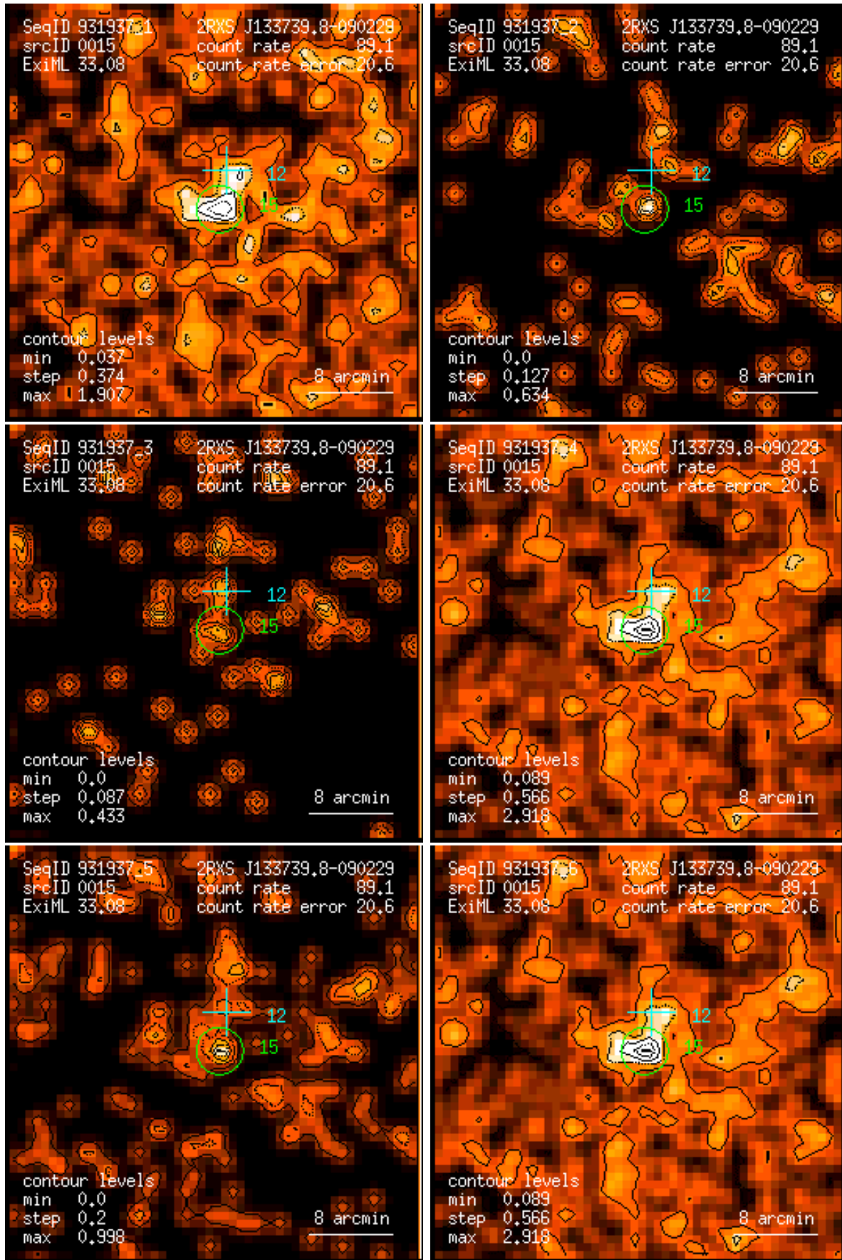
Figure 15: RASS 931937: detection 0015: band rate images, Gaussian filter: (1) PSPC channels 11 – 41, (2) 52 – 90, (3) 91 – 201, (4) 11 – 235, (5) 52 – 201, (6) 11 – 201. Broad band rates in counts/ks. Band rate contour levels in counts/ks/arcmin 2 .
