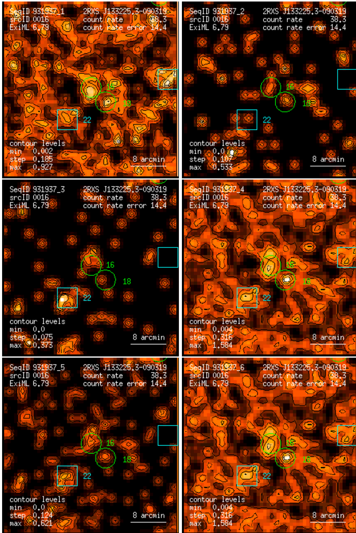
Figure 16: RASS 931937: detection 0016: band rate images, Gaussian filter: (1) PSPC channels 11 – 41, (2) 52 – 90, (3) 91 – 201, (4) 11 – 235, (5) 52 – 201, (6) 11 – 201. Broad band rates in counts/ks. Band rate contour levels in counts/ks/arcmin 2 .
