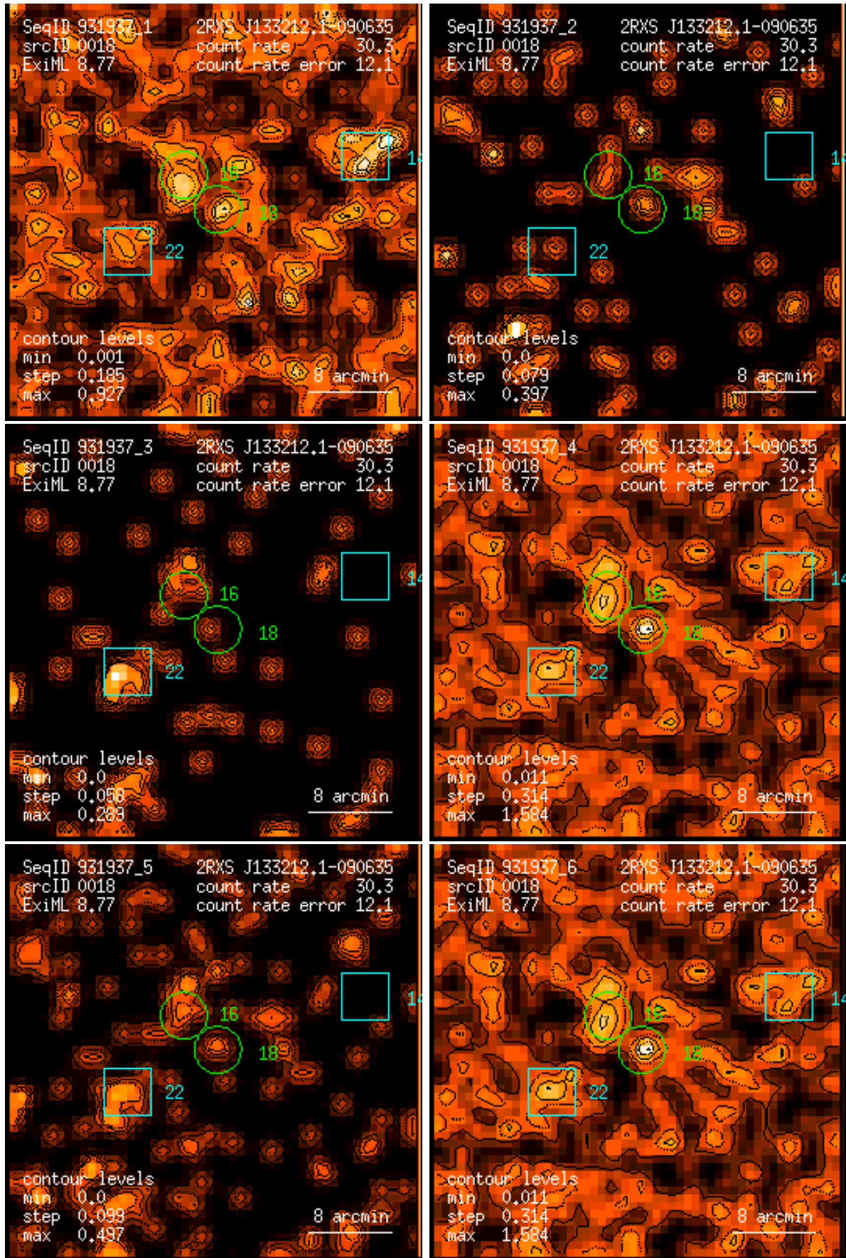
Figure 18: RASS 931937: detection 0018: band rate images, Gaussian filter: (1) PSPC channels 11 – 41, (2) 52 – 90, (3) 91 – 201, (4) 11 – 235, (5) 52 – 201, (6) 11 – 201. Broad band rates in counts/ks. Band rate contour levels in counts/ks/arcmin 2 .
