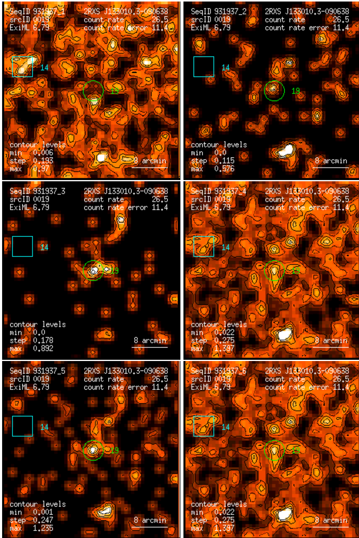
Figure 19: RASS 931937: detection 0019: band rate images, Gaussian filter: (1) PSPC channels 11 – 41, (2) 52 – 90, (3) 91 – 201, (4) 11 – 235, (5) 52 – 201, (6) 11 – 201. Broad band rates in counts/ks. Band rate contour levels in counts/ks/arcmin 2 .
