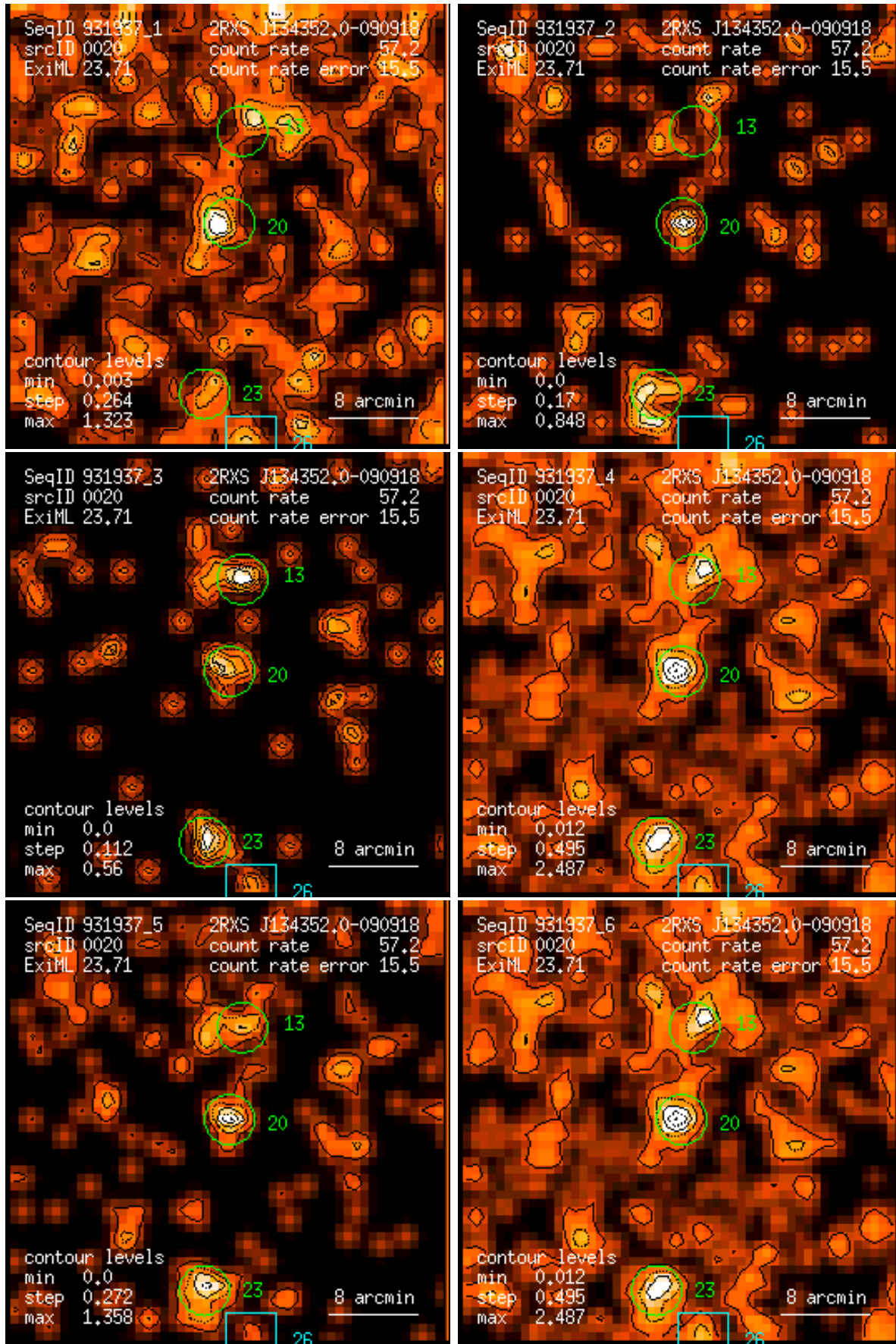
Figure 20: RASS 931937: detection 0020: band rate images, Gaussian filter: (1) PSPC channels 11 – 41, (2) 52 – 90, (3) 91 – 201, (4) 11 – 235, (5) 52 – 201, (6) 11 – 201. Broad band rates in counts/ks. Band rate contour levels in counts/ks/arcmin 2 .
