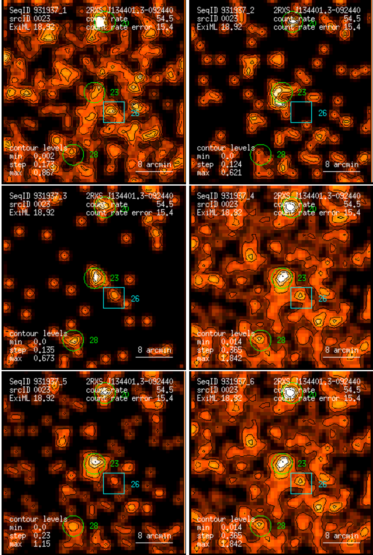
Figure 23: RASS 931937: detection 0023: band rate images, Gaussian filter: (1) PSPC channels 11 – 41, (2) 52 – 90, (3) 91 – 201, (4) 11 – 235, (5) 52 – 201, (6) 11 – 201. Broad band rates in counts/ks. Band rate contour levels in counts/ks/arcmin 2 .
