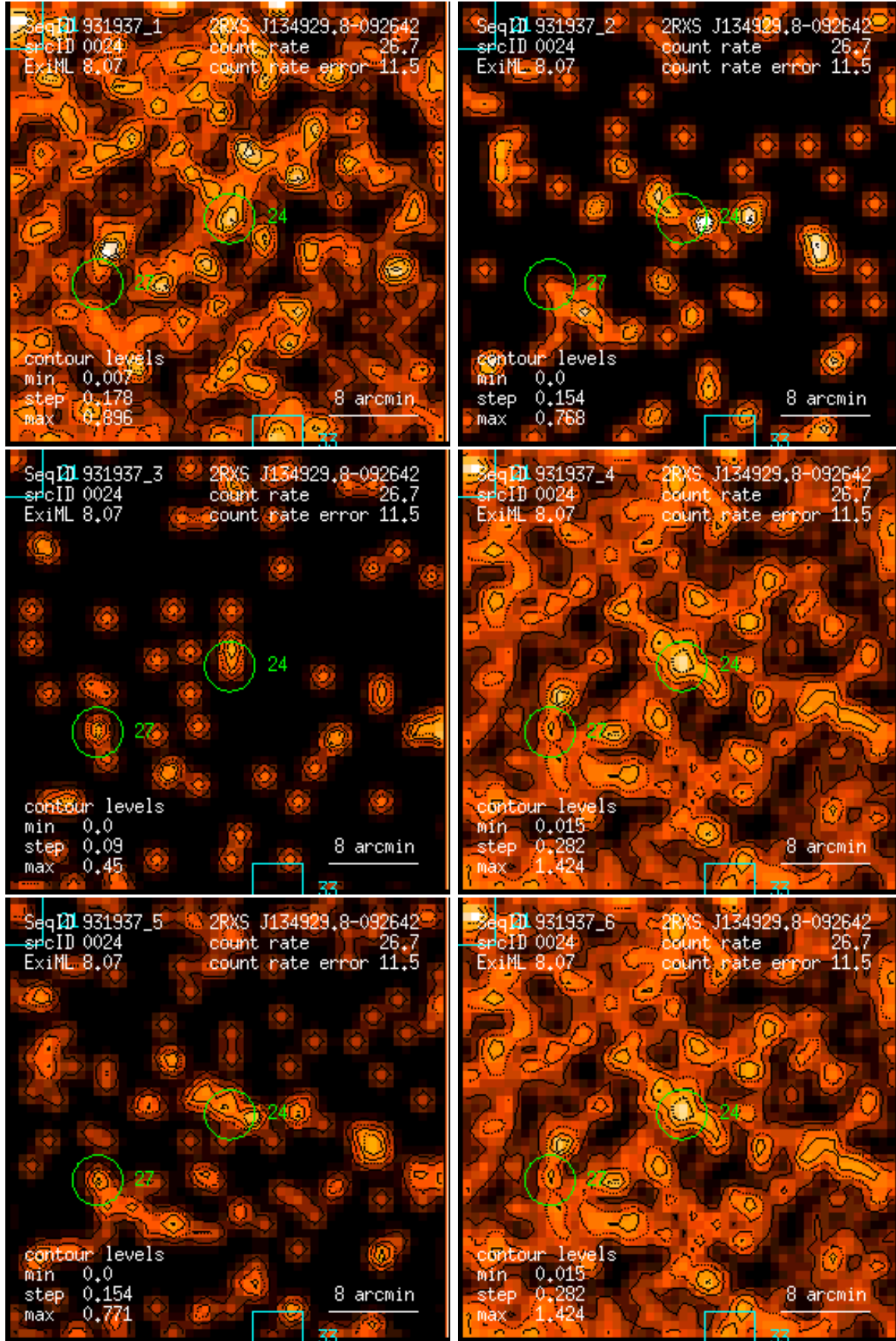
Figure 24: RASS 931937: detection 0024: band rate images, Gaussian filter: (1) PSPC channels 11 – 41, (2) 52 – 90, (3) 91 – 201, (4) 11 – 235, (5) 52 – 201, (6) 11 – 201. Broad band rates in counts/ks. Band rate contour levels in counts/ks/arcmin 2 .
