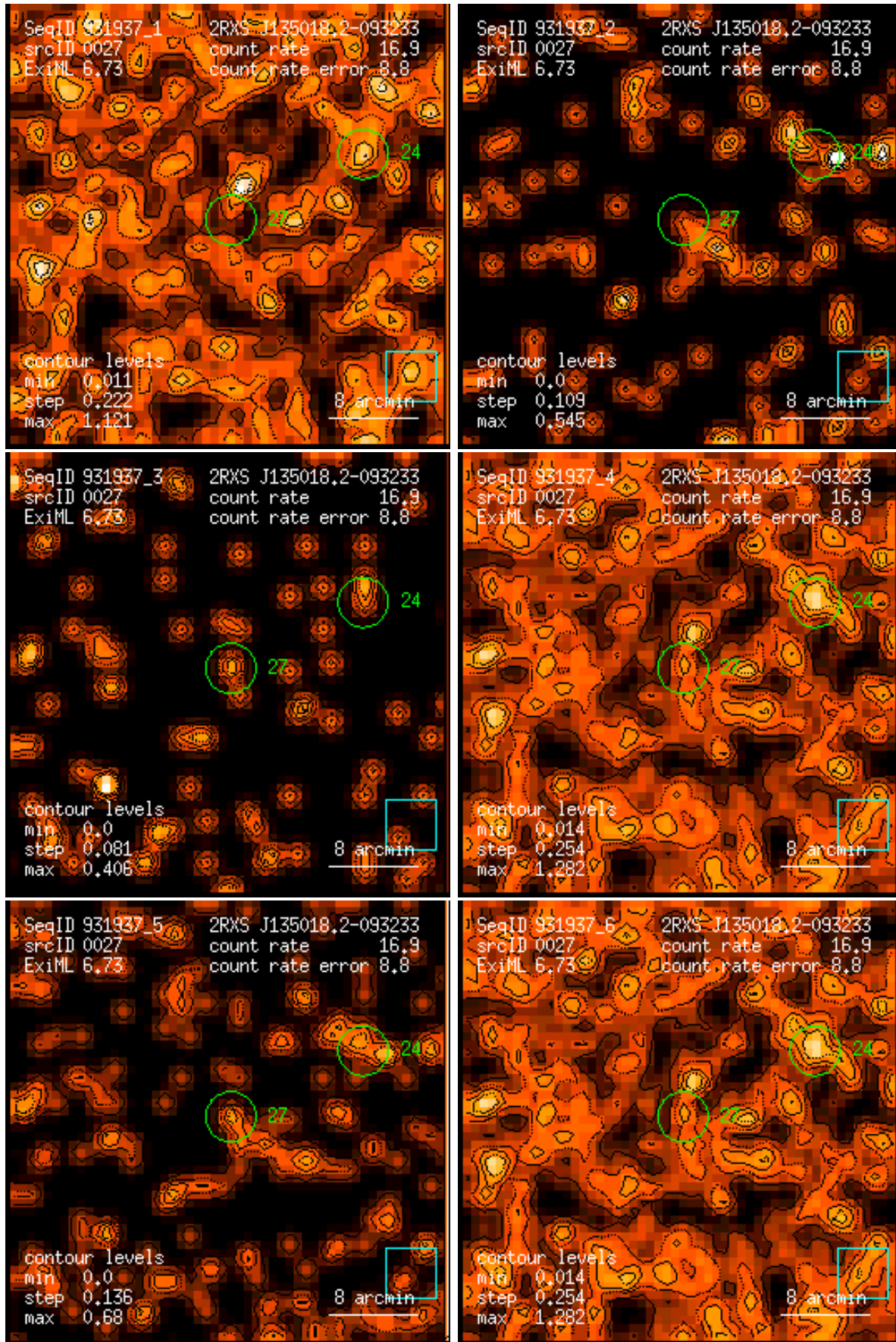
Figure 27: RASS 931937: detection 0027: band rate images, Gaussian filter: (1) PSPC channels 11 – 41, (2) 52 – 90, (3) 91 – 201, (4) 11 – 235, (5) 52 – 201, (6) 11 – 201. Broad band rates in counts/ks. Band rate contour levels in counts/ks/arcmin 2 .
