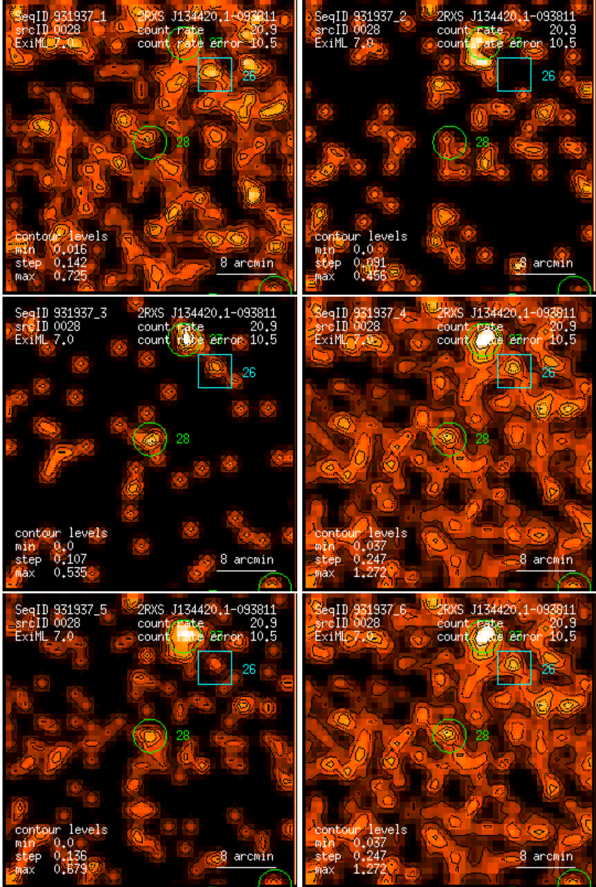
Figure 28: RASS 931937: detection 0028: band rate images, Gaussian filter: (1) PSPC channels 11 – 41, (2) 52 – 90, (3) 91 – 201, (4) 11 – 235, (5) 52 – 201, (6) 11 – 201. Broad band rates in counts/ks. Band rate contour levels in counts/ks/arcmin 2 .
