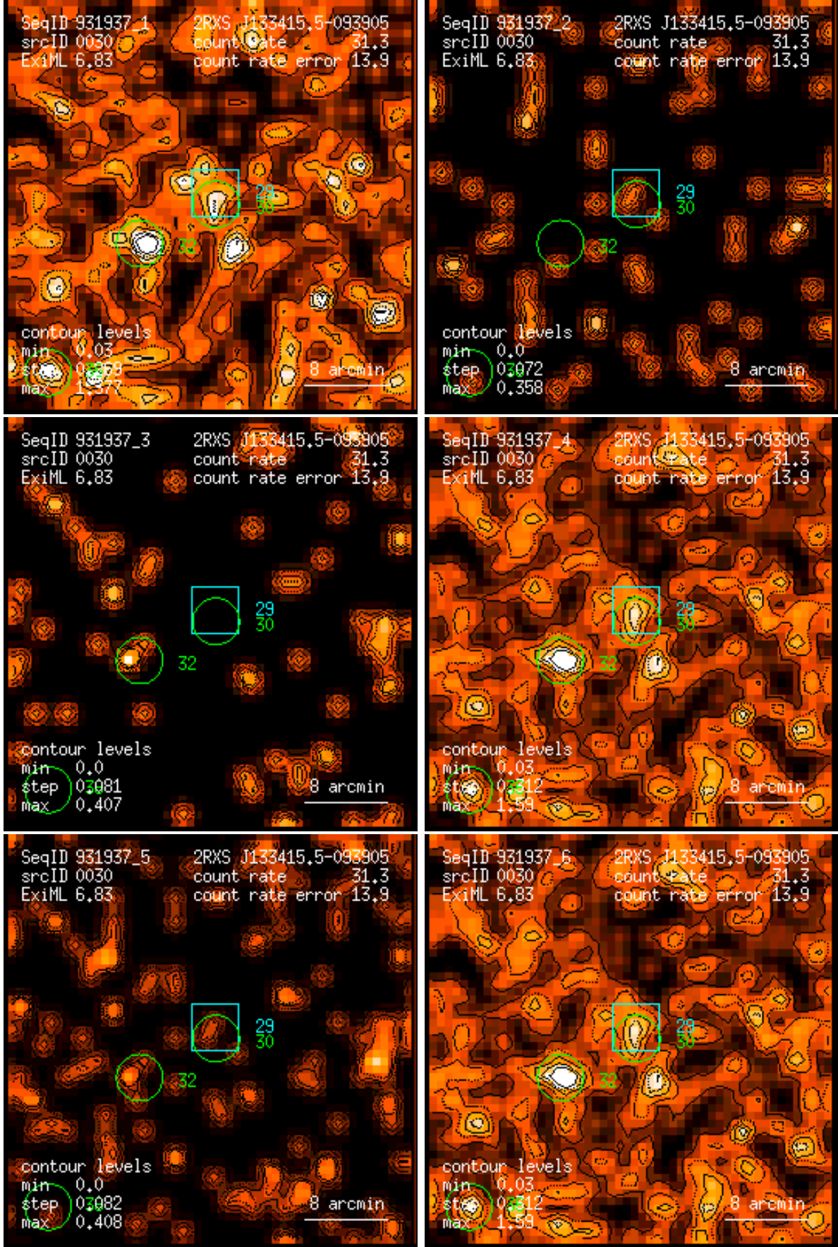
Figure 30: RASS 931937: detection 0030: band rate images, Gaussian filter: (1) PSPC channels 11 – 41, (2) 52 – 90, (3) 91 – 201, (4) 11 – 235, (5) 52 – 201, (6) 11 – 201. Broad band rates in counts/ks. Band rate contour levels in counts/ks/arcmin 2 .
