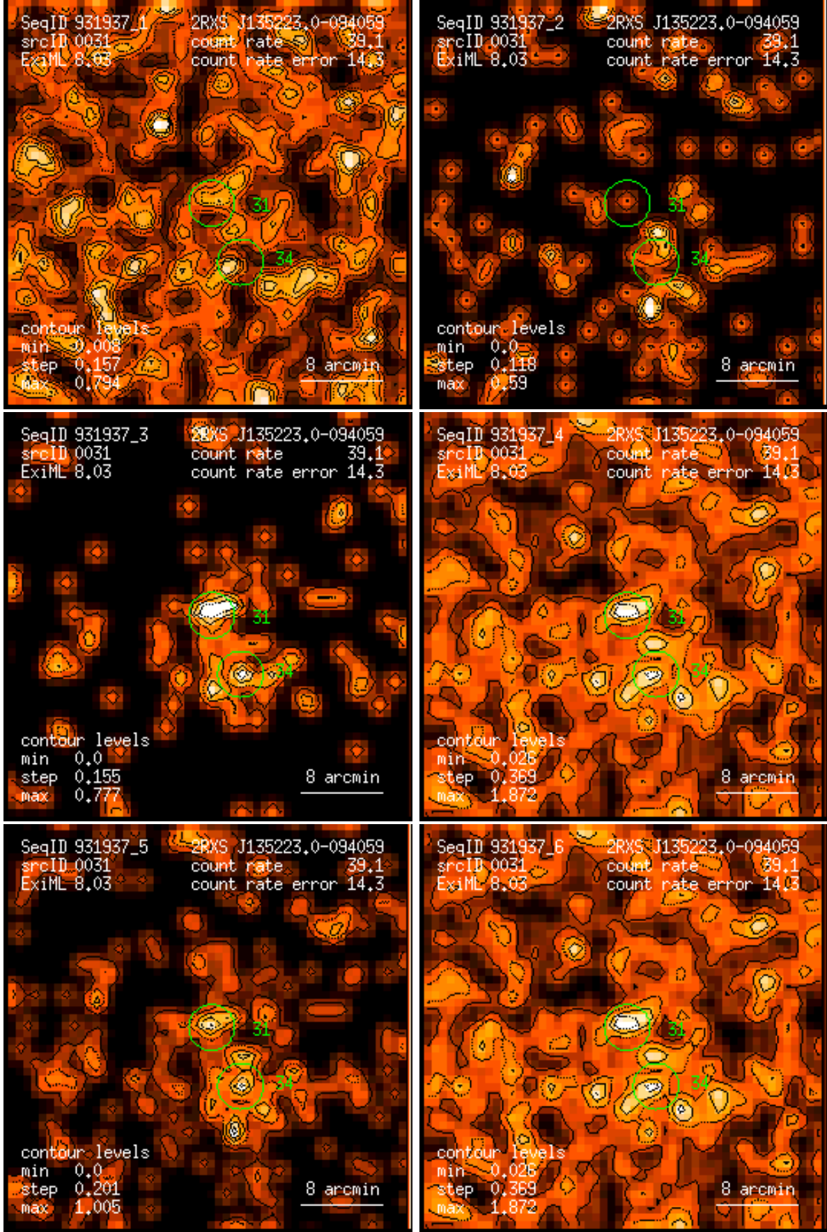
Figure 31: RASS 931937: detection 0031: band rate images, Gaussian filter: (1) PSPC channels 11 – 41, (2) 52 – 90, (3) 91 – 201, (4) 11 – 235, (5) 52 – 201, (6) 11 – 201. Broad band rates in counts/ks. Band rate contour levels in counts/ks/arcmin 2 .
