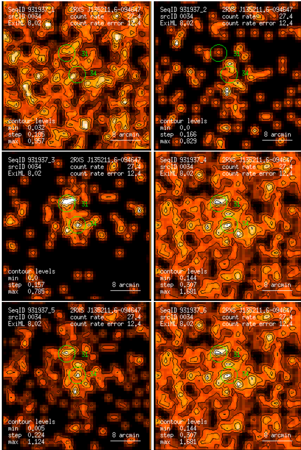
Figure 34: RASS 931937: detection 0034: band rate images, Gaussian filter: (1) PSPC channels 11 – 41, (2) 52 – 90, (3) 91 – 201, (4) 11 – 235, (5) 52 – 201, (6) 11 – 201. Broad band rates in counts/ks. Band rate contour levels in counts/ks/arcmin 2 .
