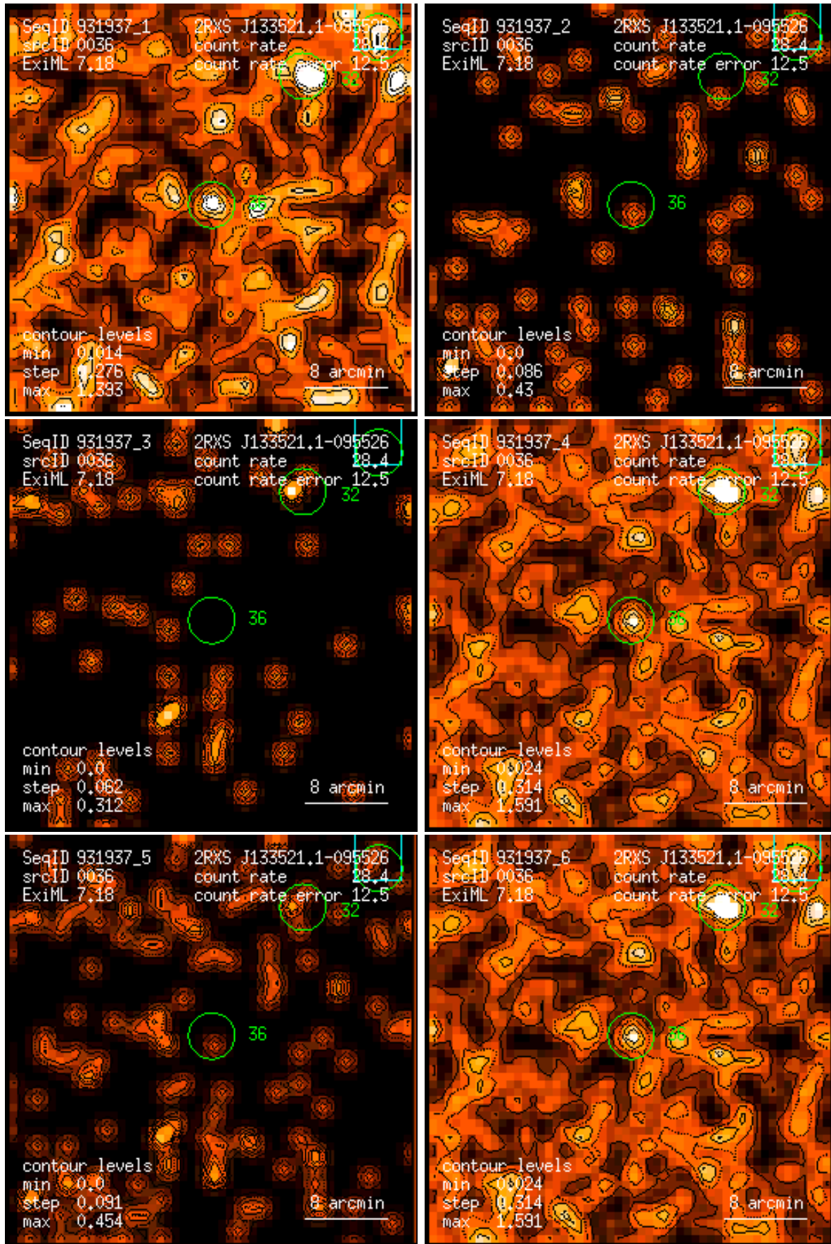
Figure 36: RASS 931937: detection 0036: band rate images, Gaussian filter: (1) PSPC channels 11 – 41, (2) 52 – 90, (3) 91 – 201, (4) 11 – 235, (5) 52 – 201, (6) 11 – 201. Broad band rates in counts/ks. Band rate contour levels in counts/ks/arcmin 2 .
