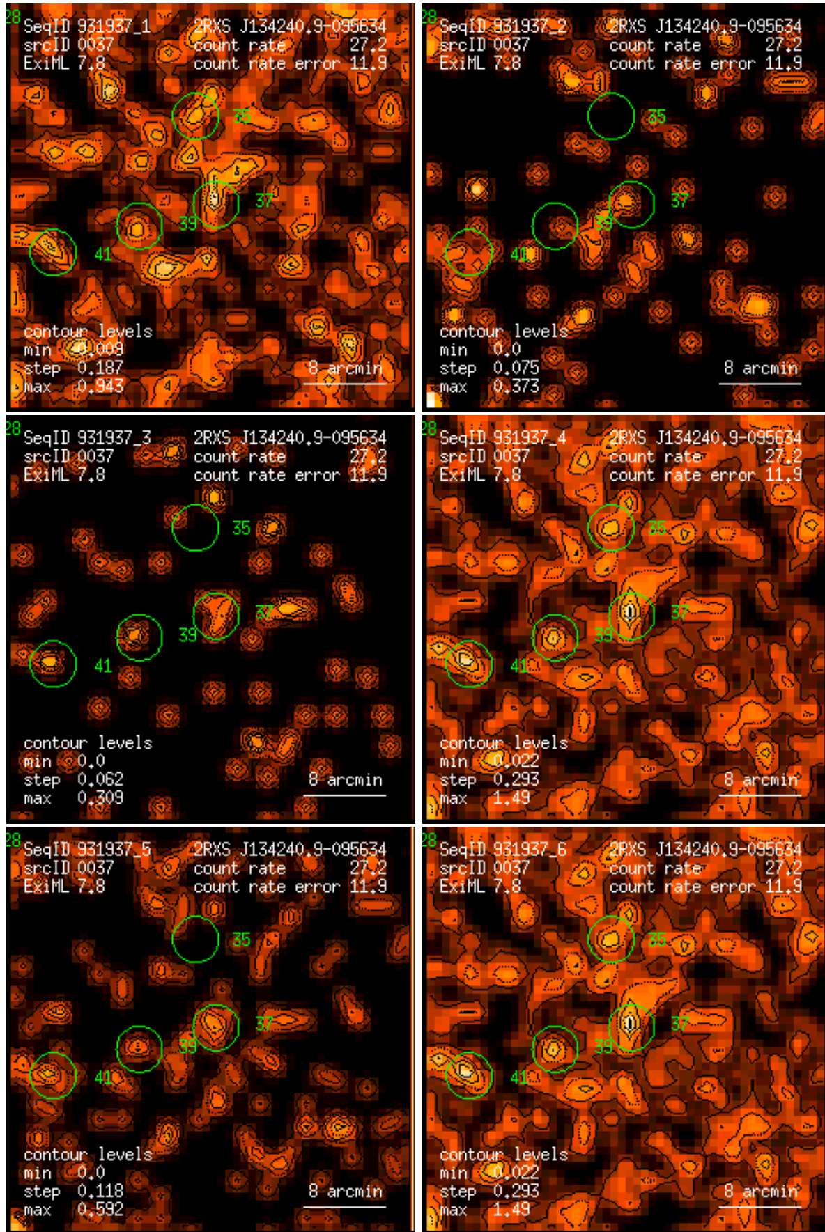
Figure 37: RASS 931937: detection 0037: band rate images, Gaussian filter: (1) PSPC channels 11 – 41, (2) 52 – 90, (3) 91 – 201, (4) 11 – 235, (5) 52 – 201, (6) 11 – 201. Broad band rates in counts/ks. Band rate contour levels in counts/ks/arcmin 2 .
